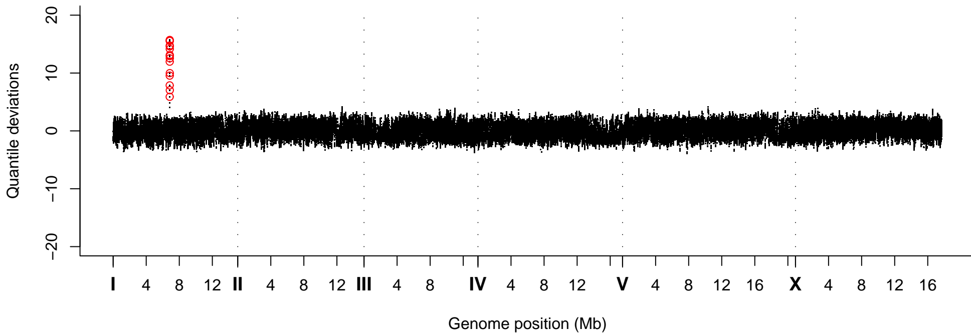
Quantile Deviations, Strain VC40670
