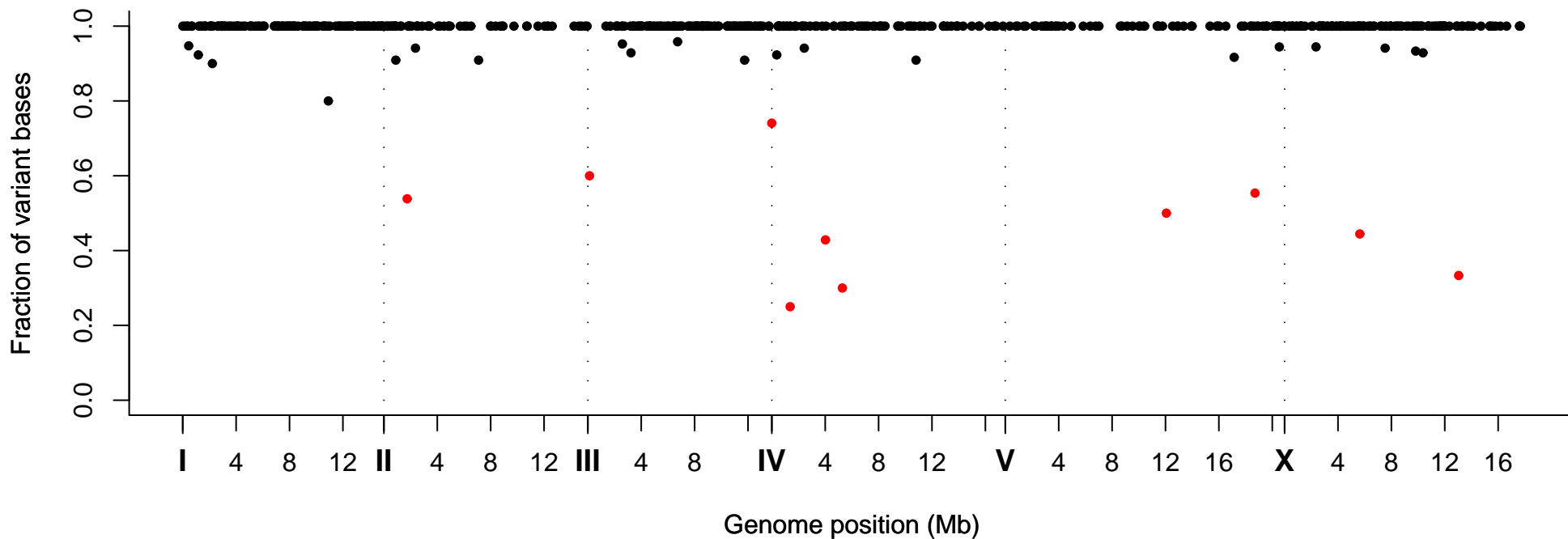
Fraction of Variant Bases at Position, Strain VC40670
