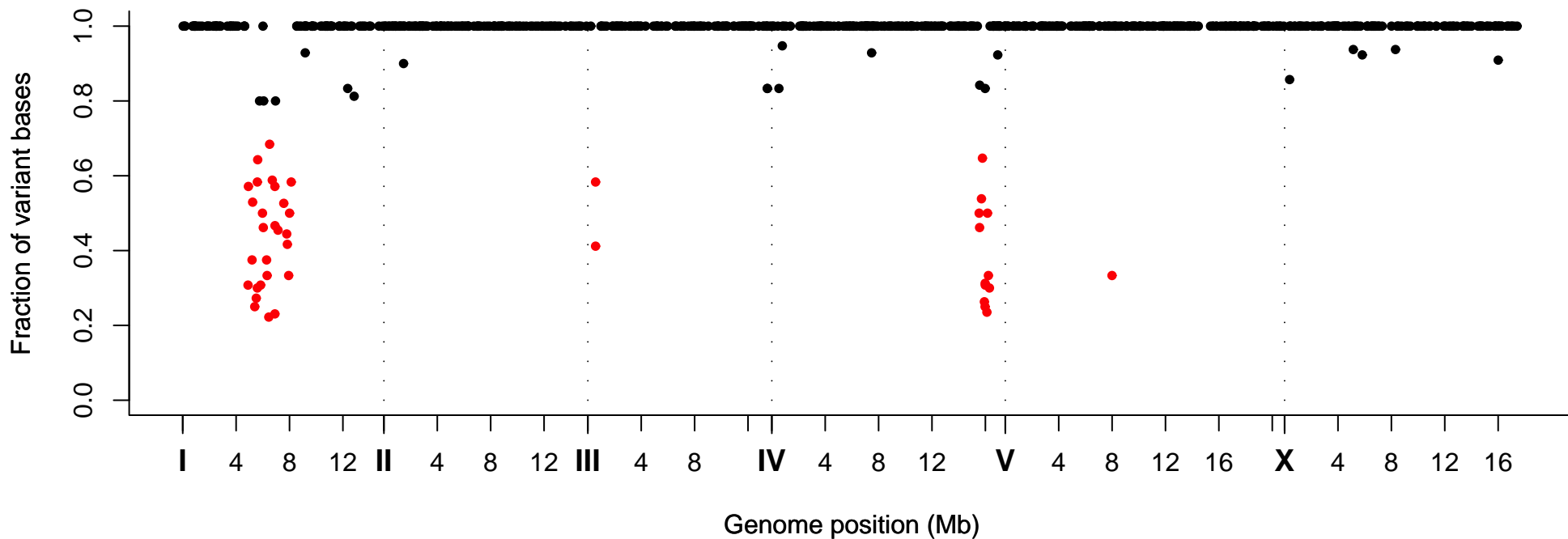
Fraction of Variant Bases at Position, Strain VC40690
