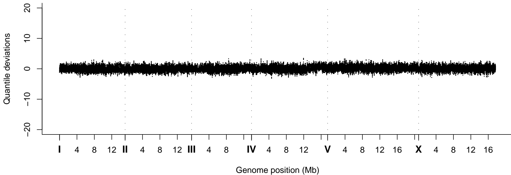
Quantile Deviations, Strain VC40690
