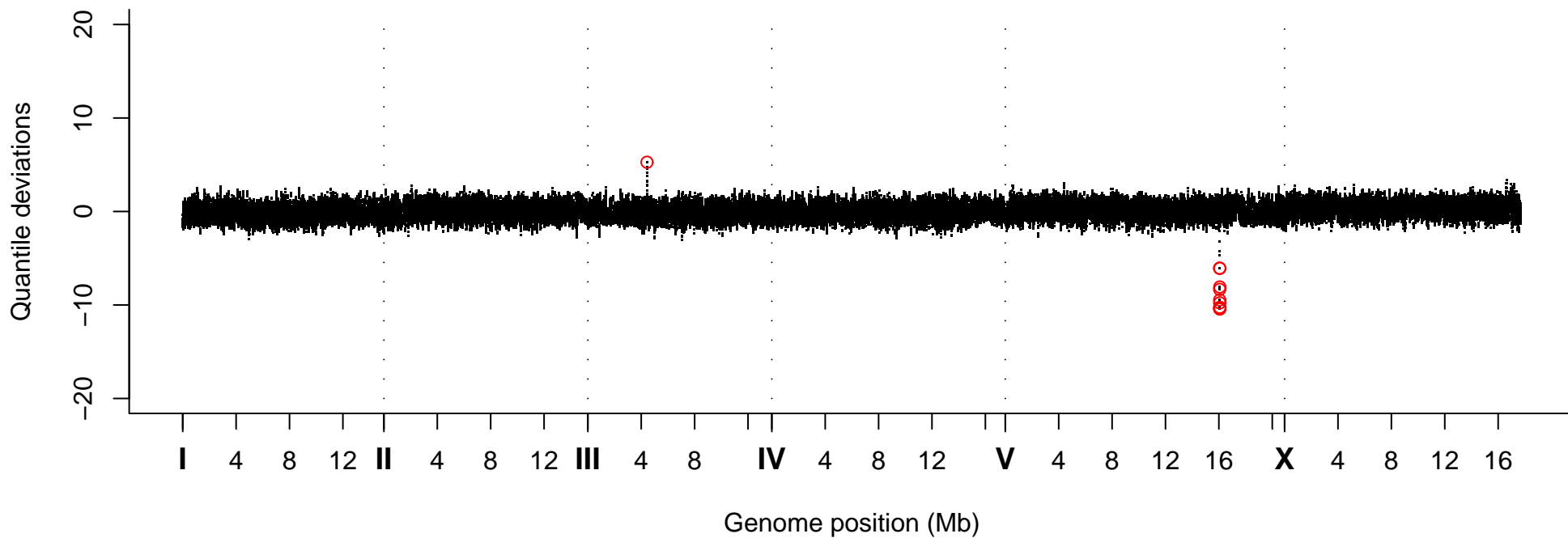
Quantile Deviations, Strain VC40691
