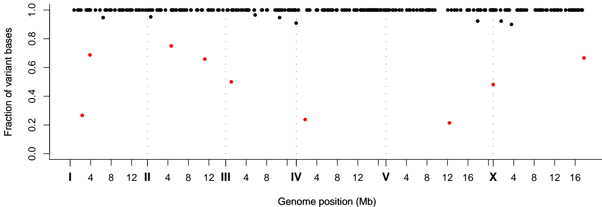
Fraction of Variant Bases at Position, Strain VC40691
