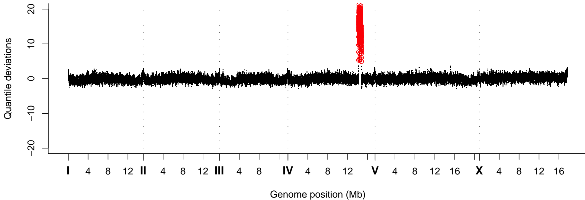
Quantile Deviations, Strain VC40693
