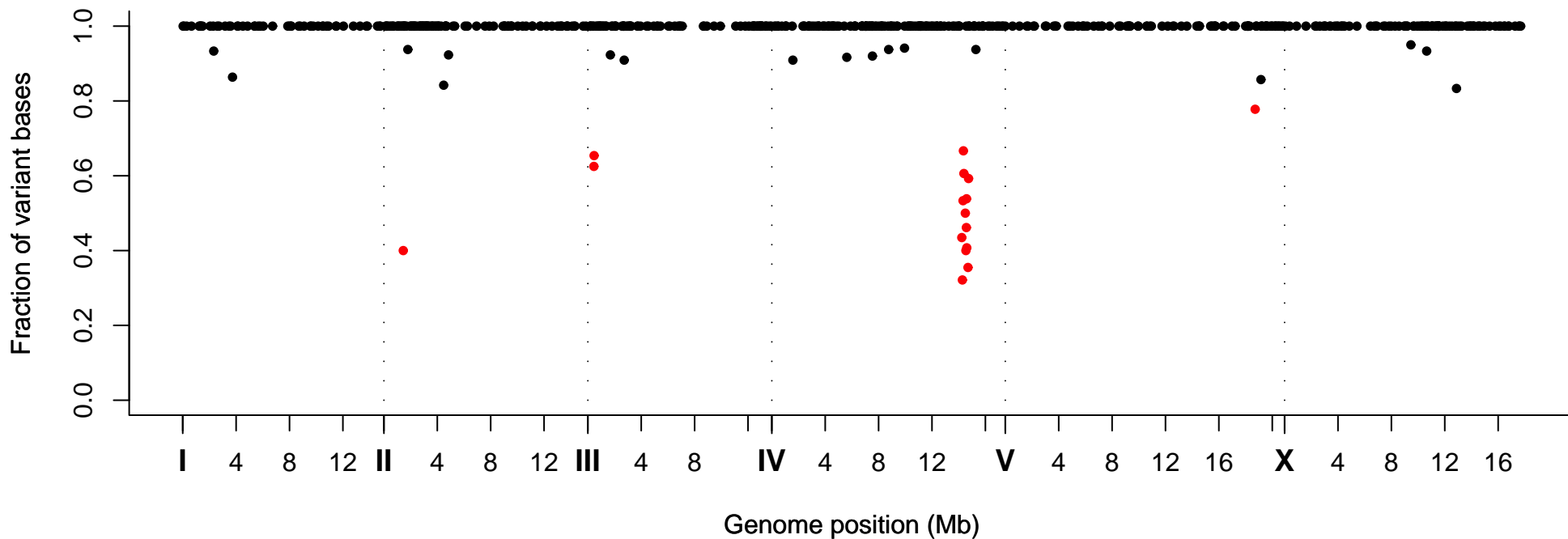
Fraction of Variant Bases at Position, Strain VC40693
