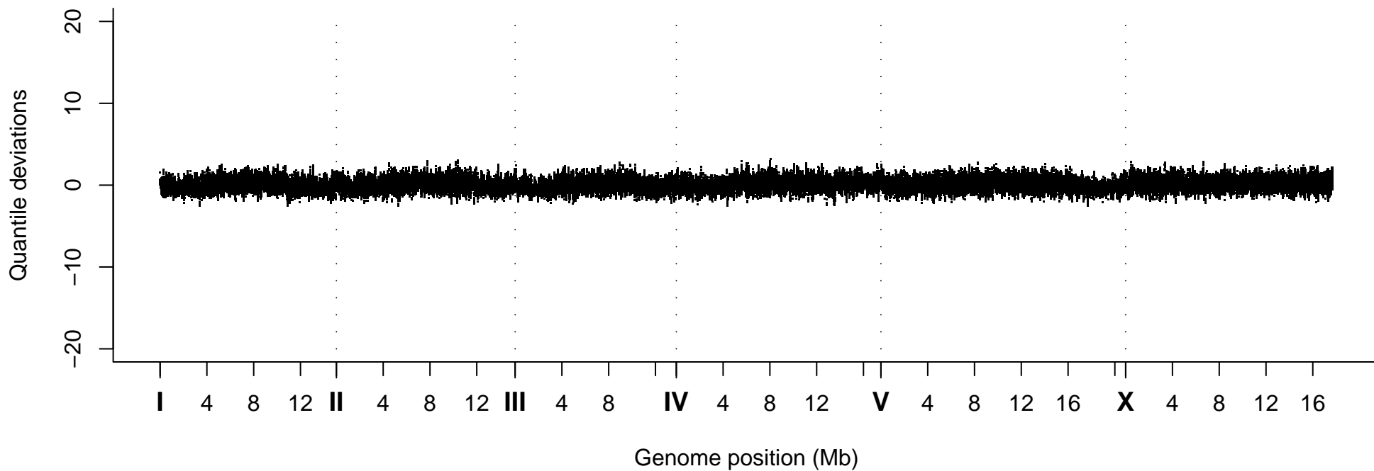
Quantile Deviations, Strain VC40695
