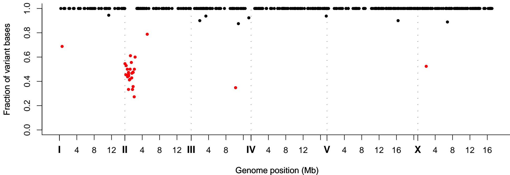
Fraction of Variant Bases at Position, Strain VC40695
