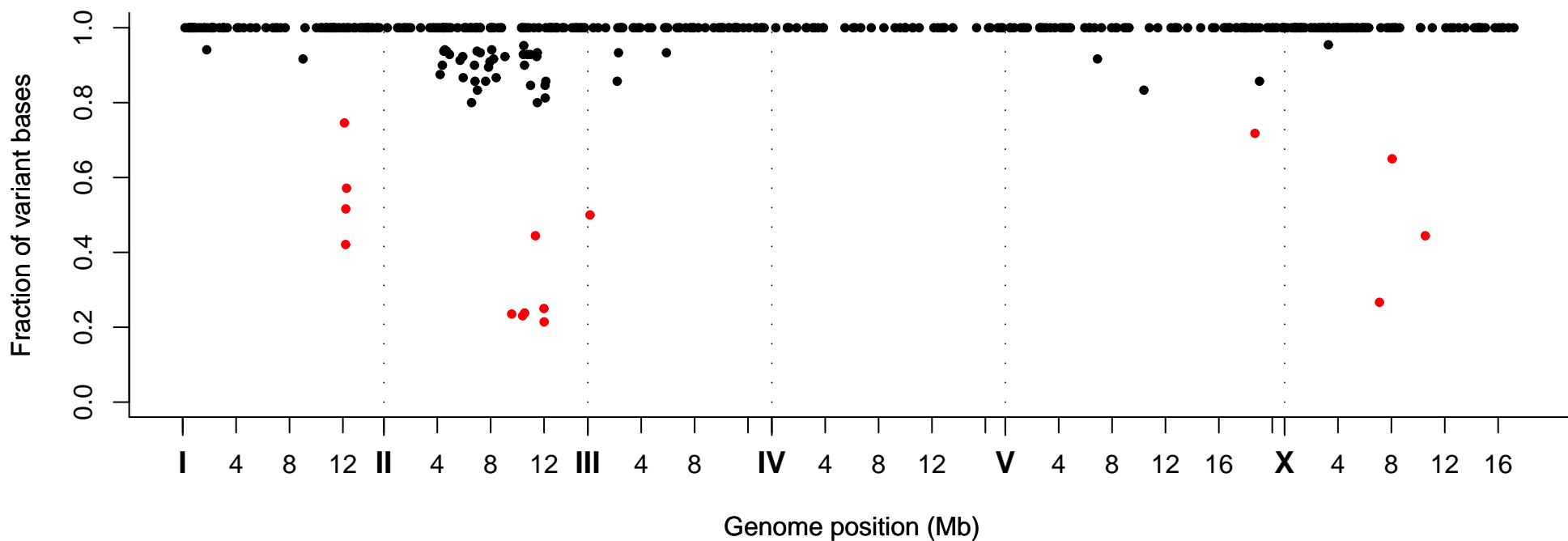
Fraction of Variant Bases at Position, Strain VC40697
