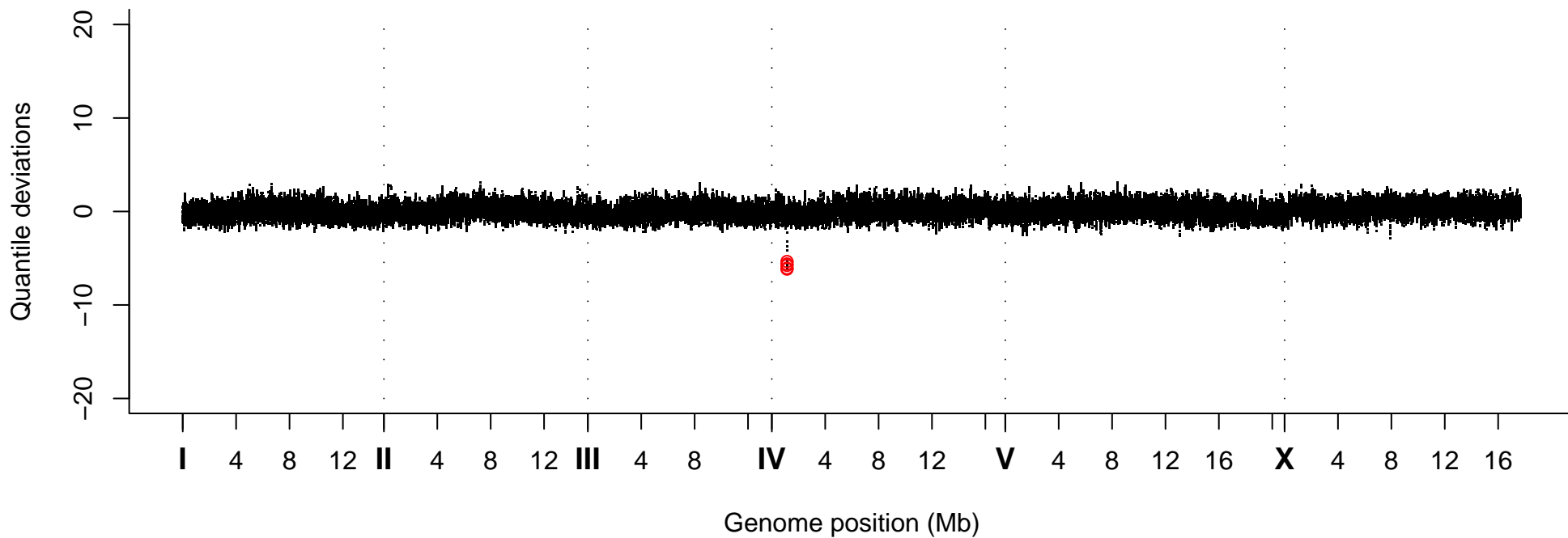
Quantile Deviations, Strain VC40698
