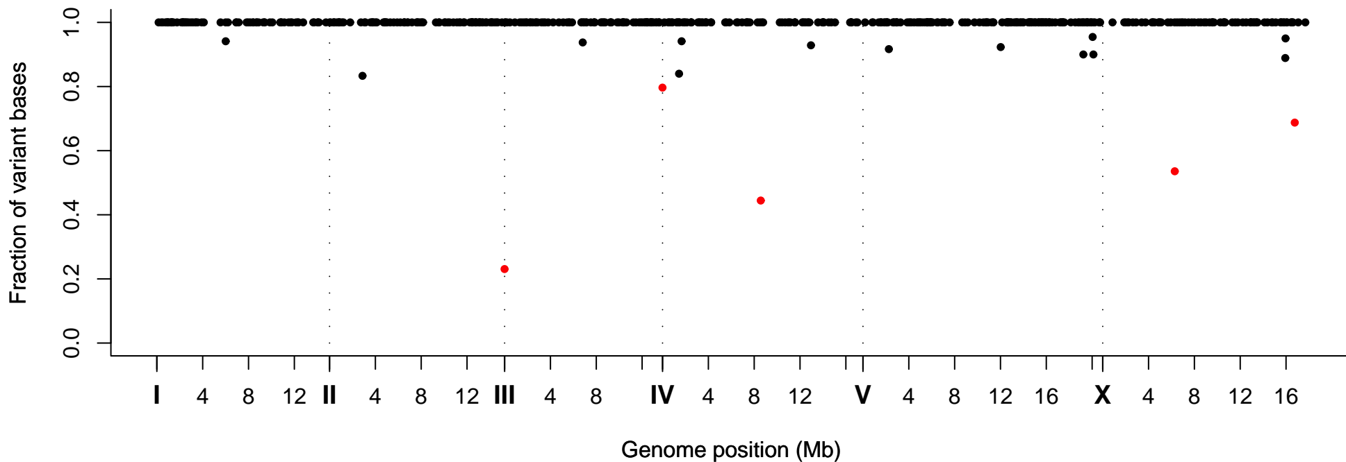
Fraction of Variant Bases at Position, Strain VC40698
