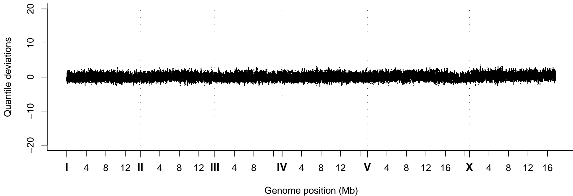
Quantile Deviations, Strain VC40706
