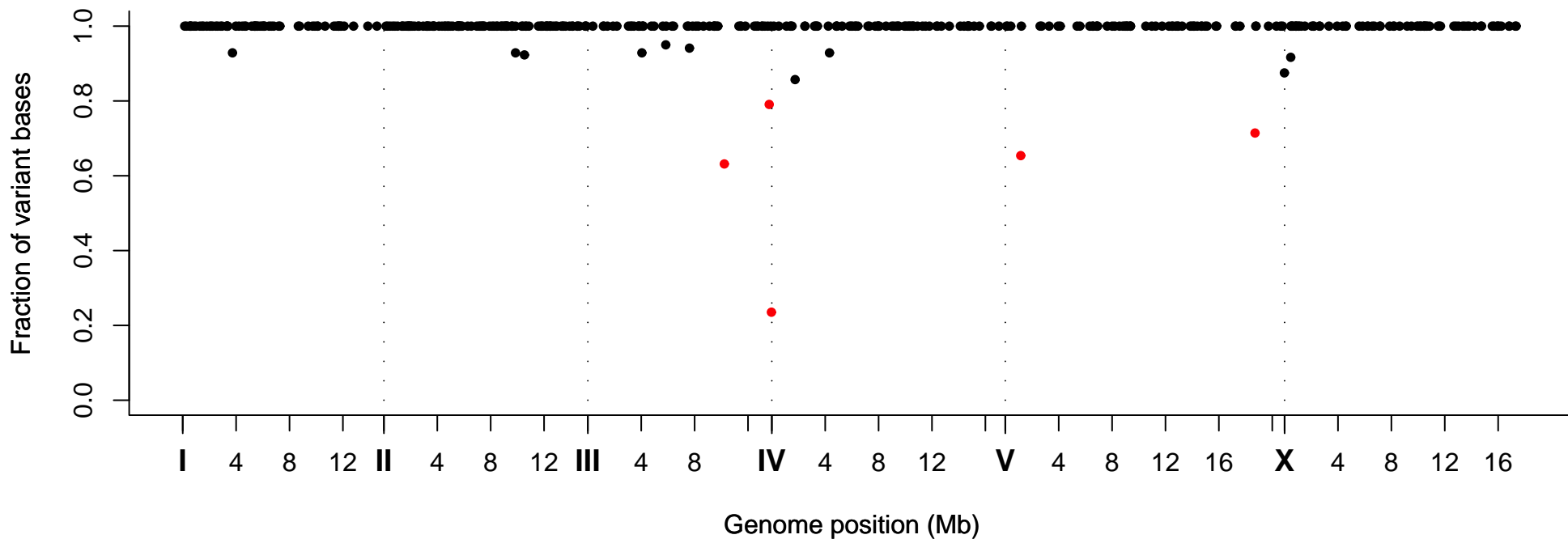
Fraction of Variant Bases at Position, Strain VC40706
