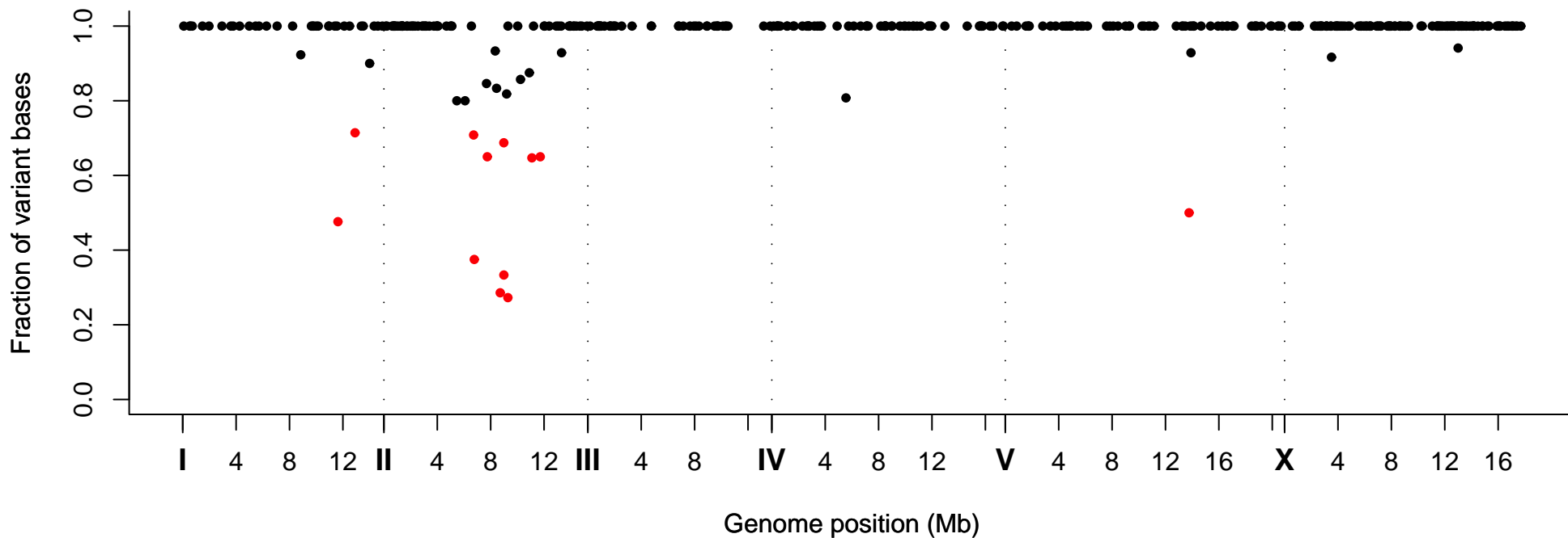
Fraction of Variant Bases at Position, Strain VC40711
