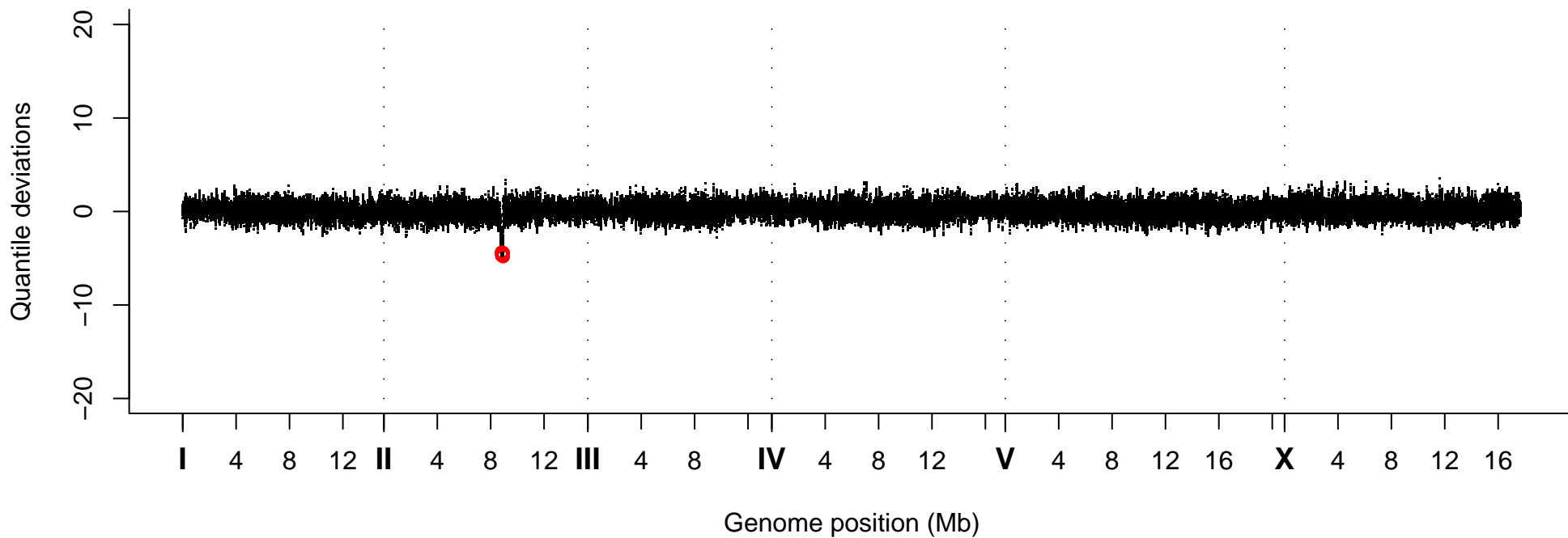
Quantile Deviations, Strain VC40711
