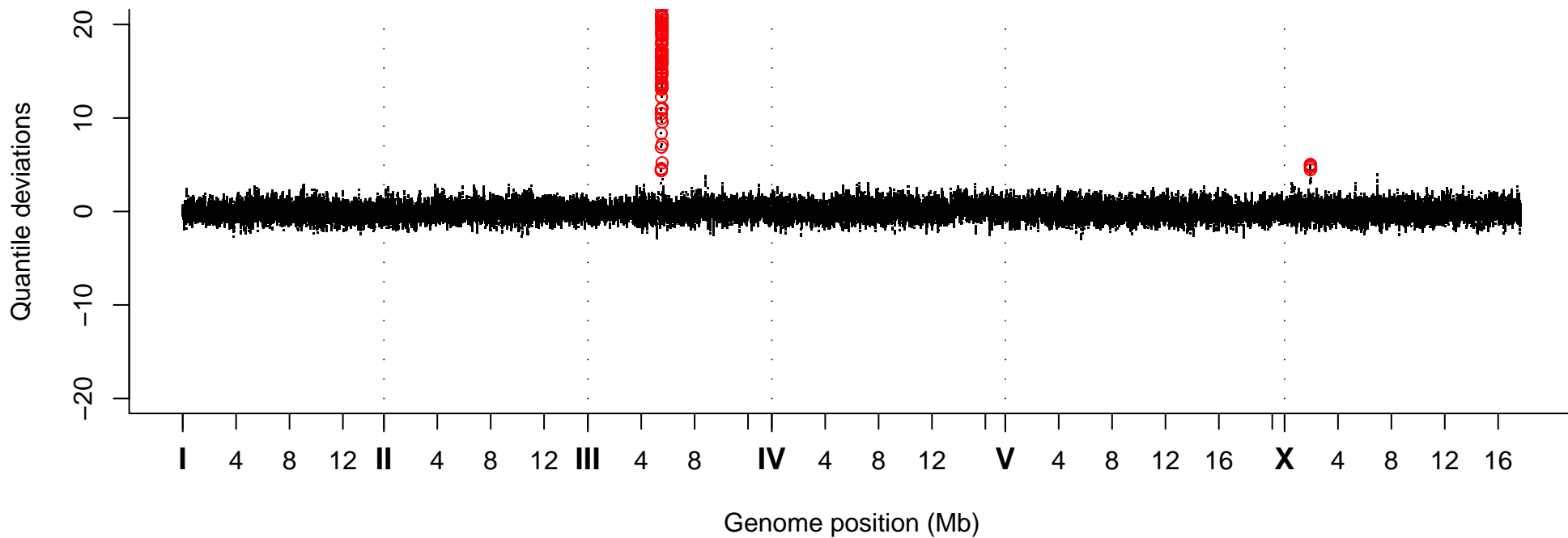
Quantile Deviations, Strain VC40713
