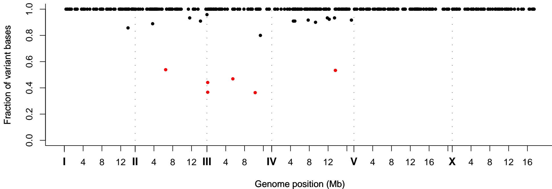
Fraction of Variant Bases at Position, Strain VC40713
