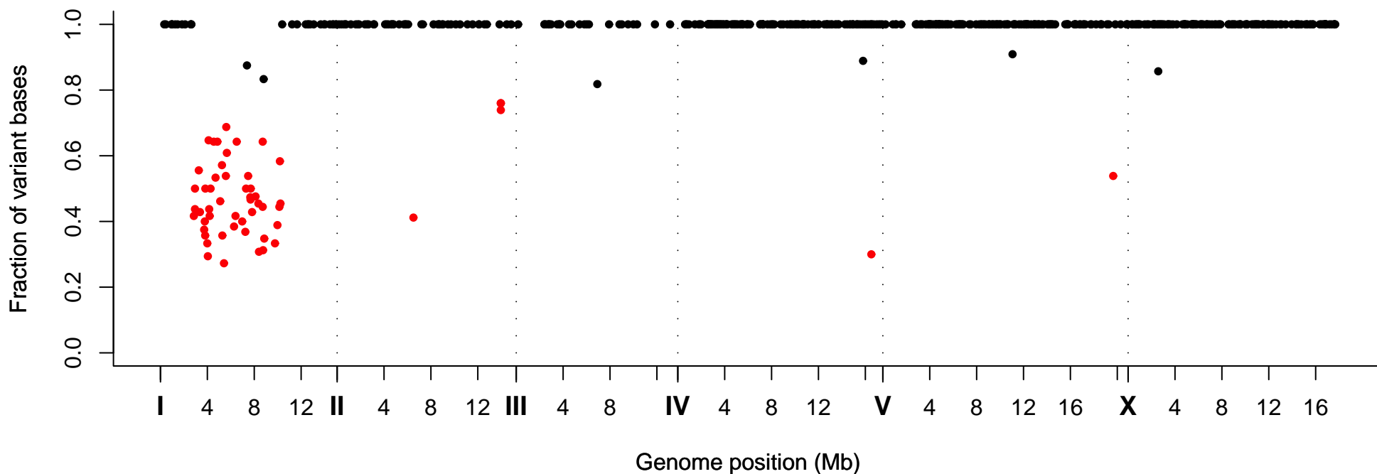
Fraction of Variant Bases at Position, Strain VC40714
