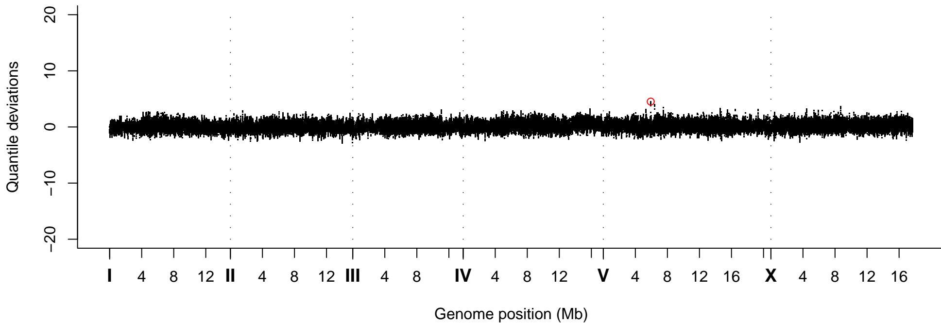
Quantile Deviations, Strain VC40714
