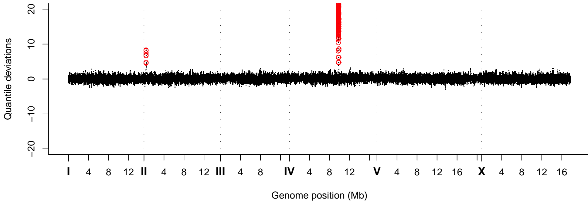
Quantile Deviations, Strain VC40722
