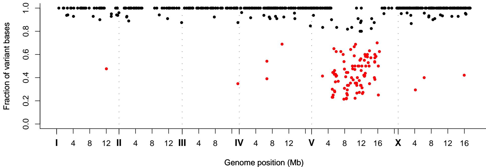
Fraction of Variant Bases at Position, Strain VC40722
