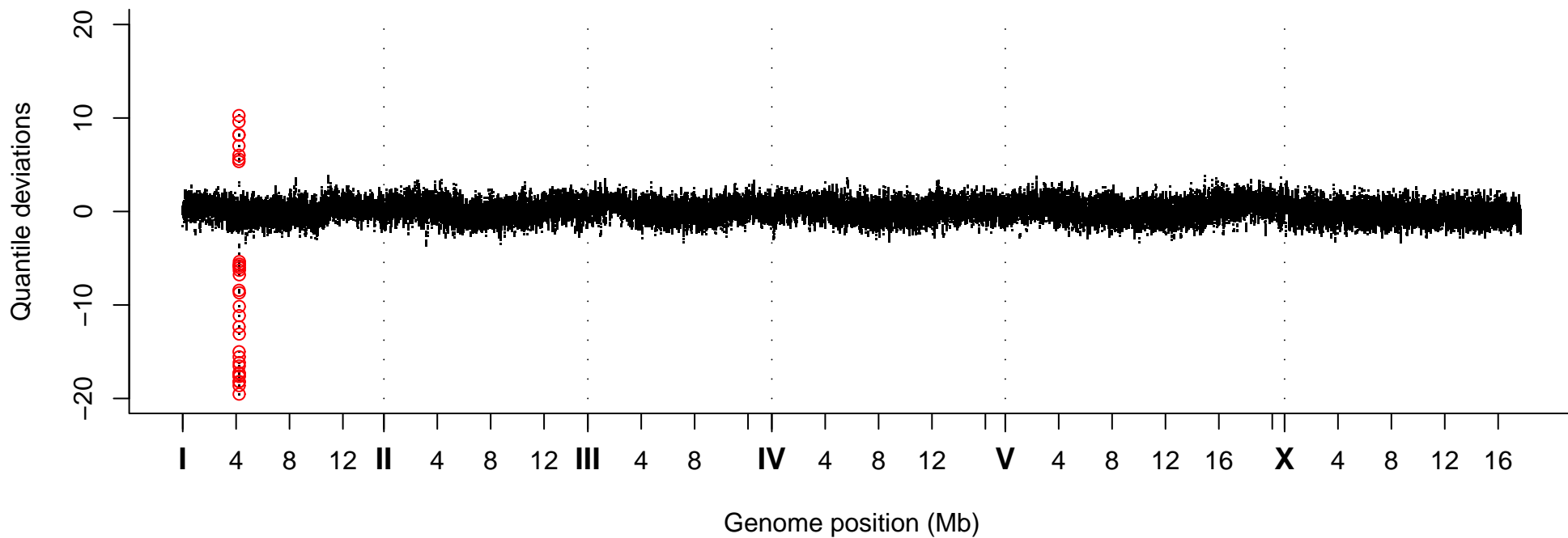
Quantile Deviations, Strain VC40727
