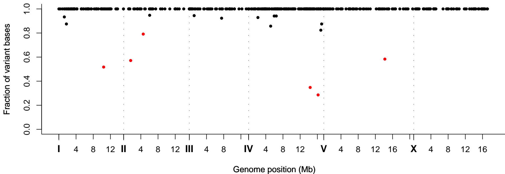
Fraction of Variant Bases at Position, Strain VC40727
