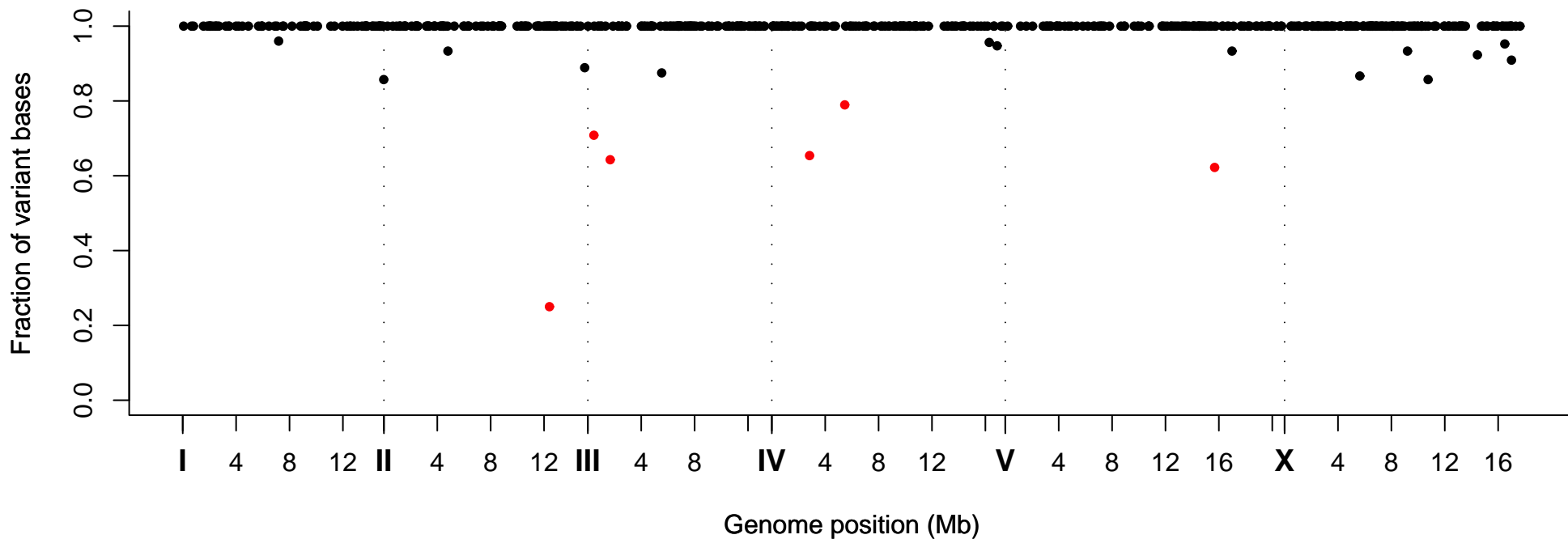
Fraction of Variant Bases at Position, Strain VC40732
