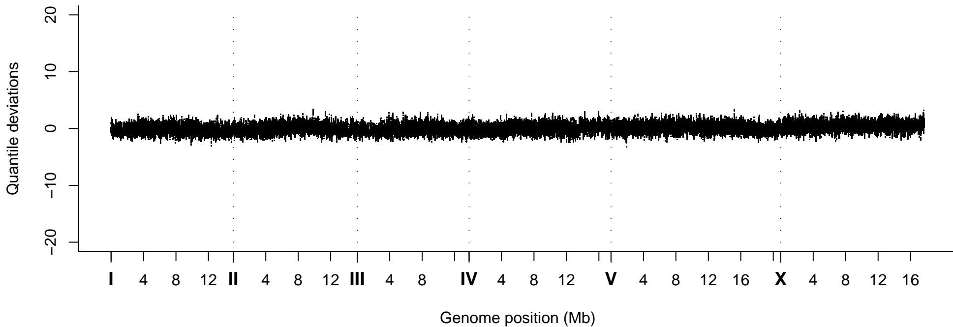
Quantile Deviations, Strain VC40732
