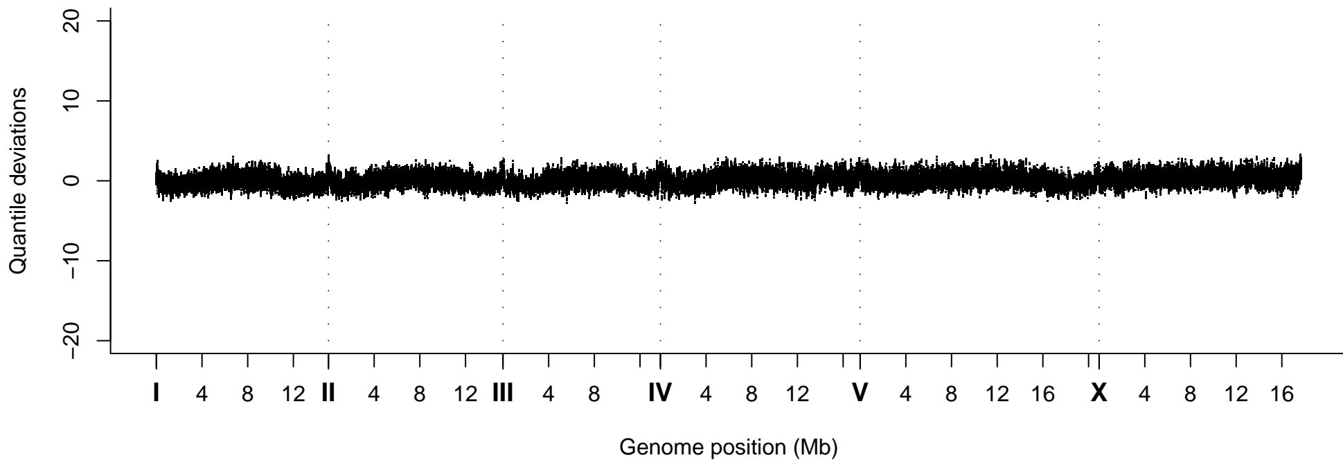
Quantile Deviations, Strain VC40737
