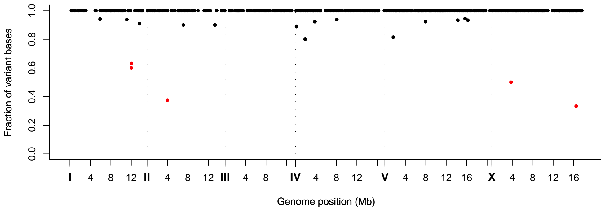
Fraction of Variant Bases at Position, Strain VC40737
