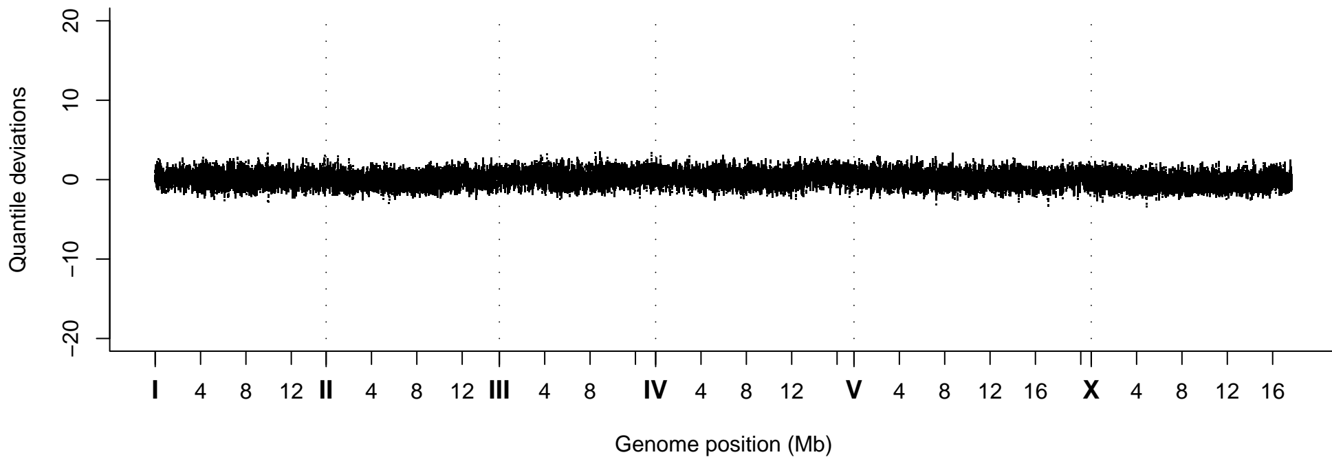
Quantile Deviations, Strain VC40740
