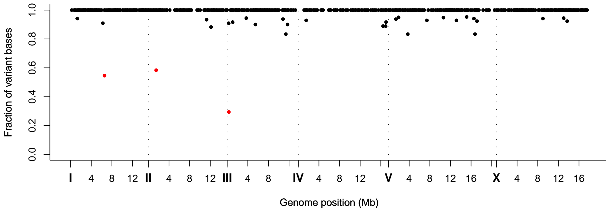
Fraction of Variant Bases at Position, Strain VC40740
