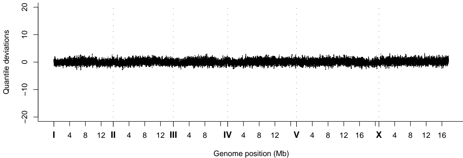
Quantile Deviations, Strain VC40741
