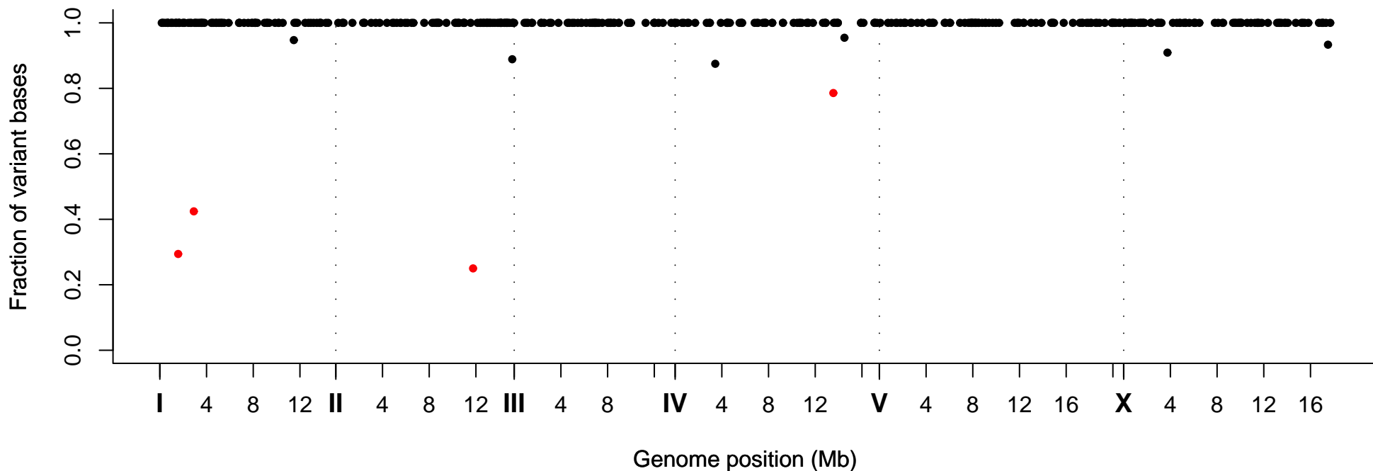
Fraction of Variant Bases at Position, Strain VC40741
