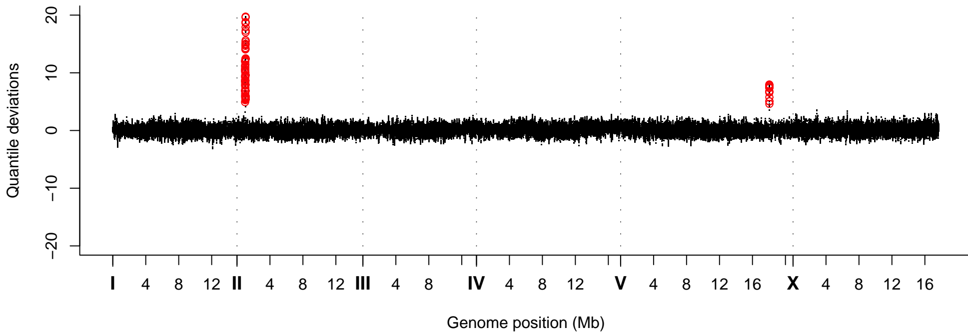
Quantile Deviations, Strain VC40743
