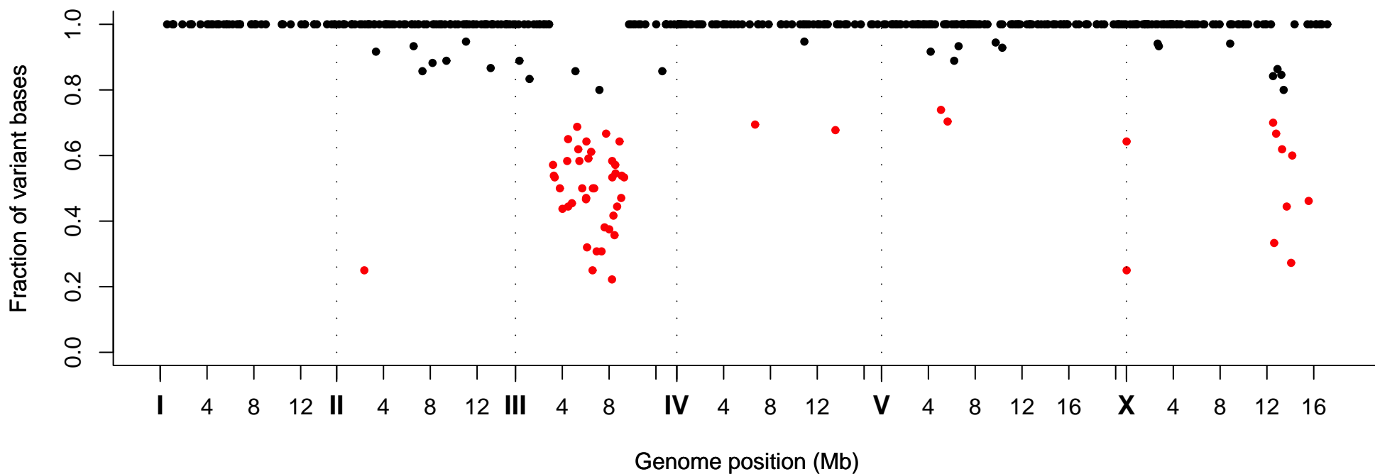
Fraction of Variant Bases at Position, Strain VC40743
