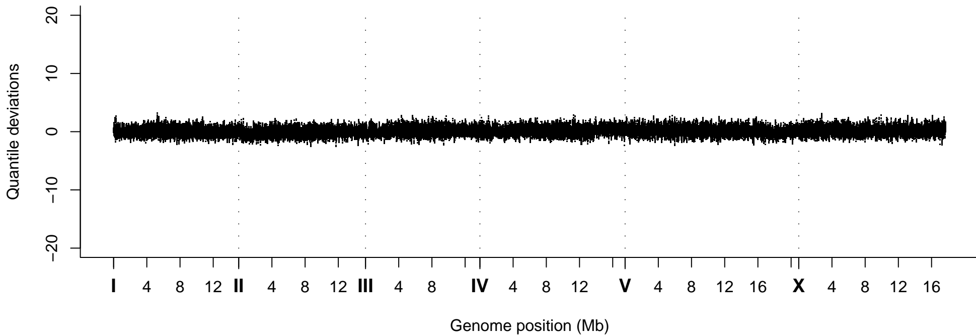
Quantile Deviations, Strain VC40748
