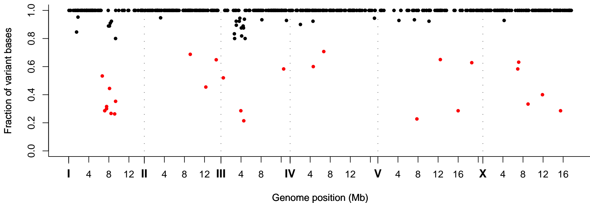
Fraction of Variant Bases at Position, Strain VC40748
