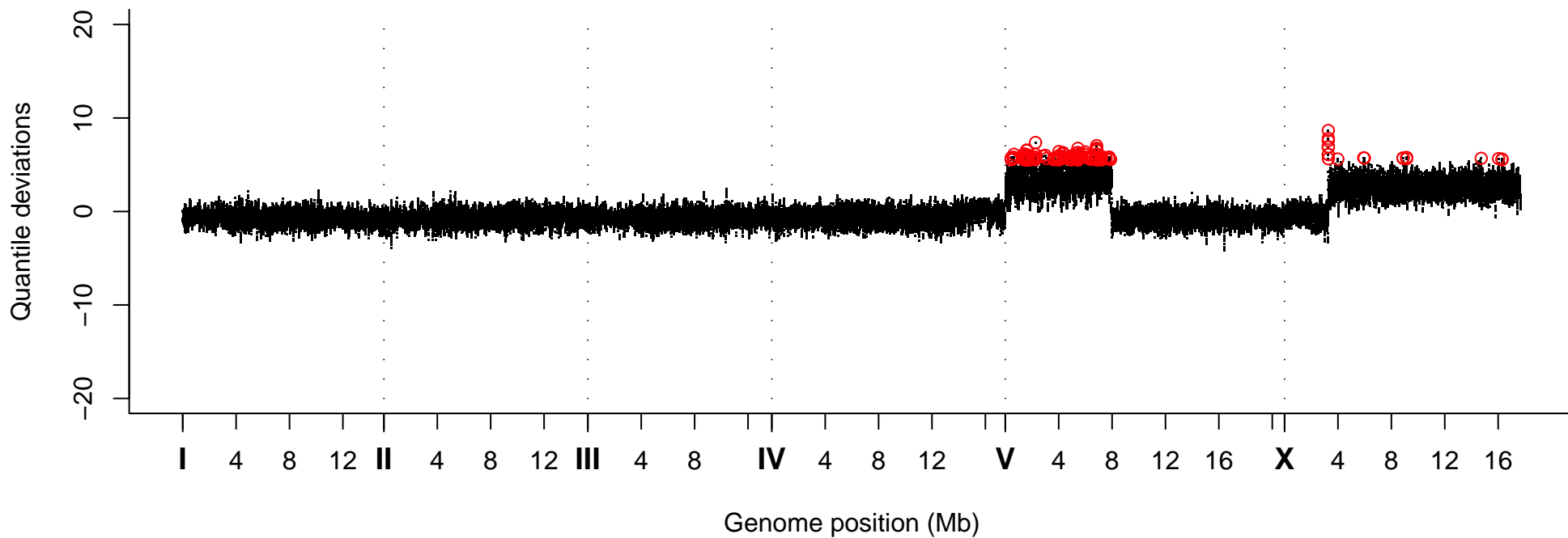
Quantile Deviations, Strain VC40750
