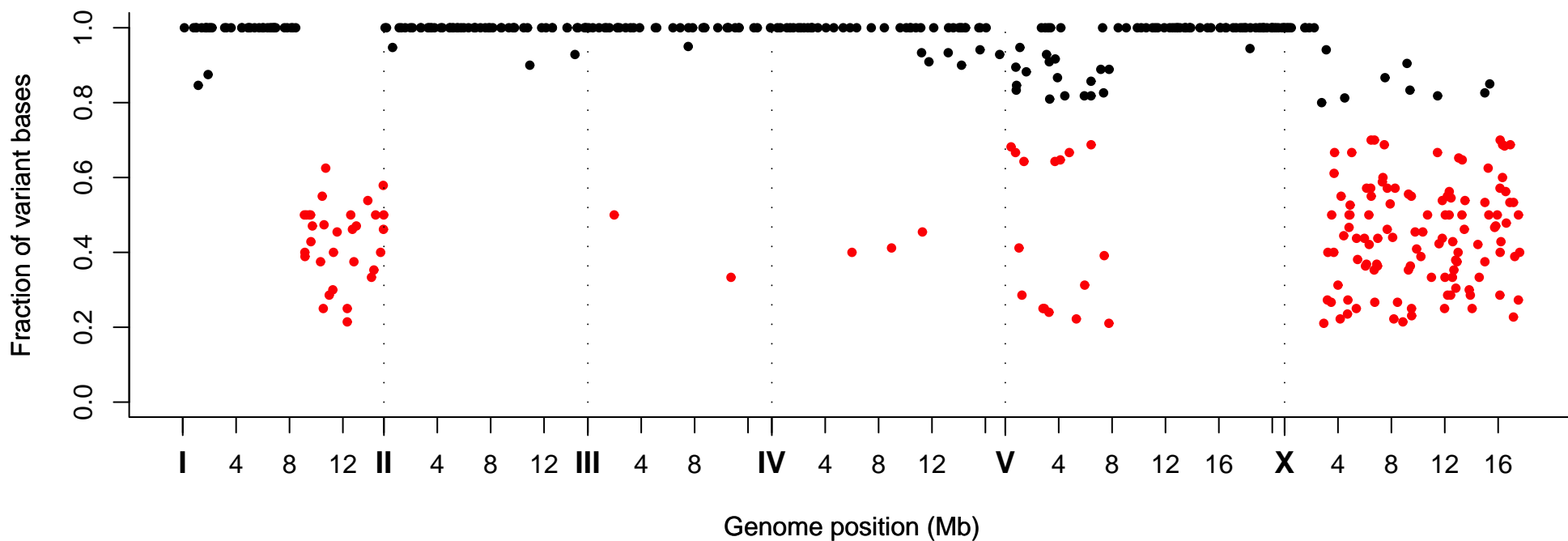
Fraction of Variant Bases at Position, Strain VC40750
