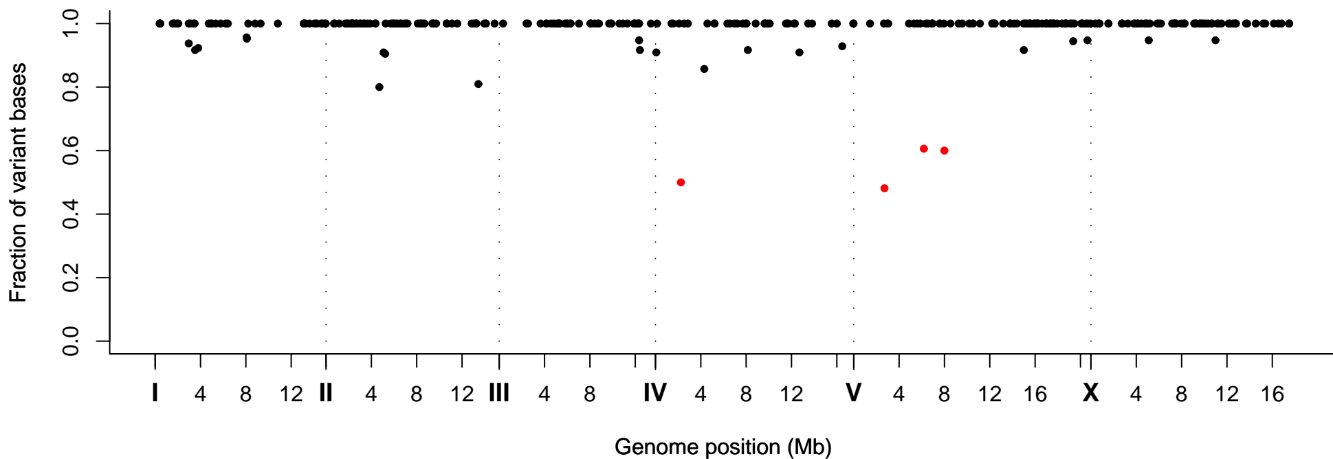
Fraction of Variant Bases at Position, Strain VC40751
