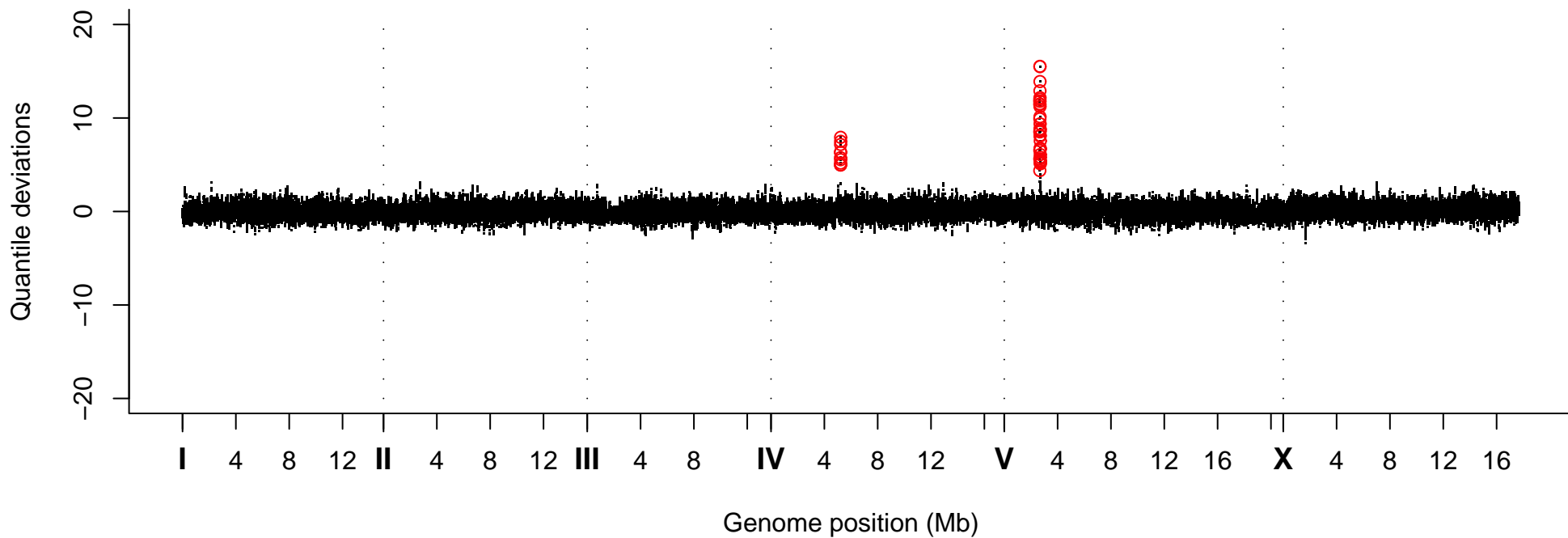
Quantile Deviations, Strain VC40751
