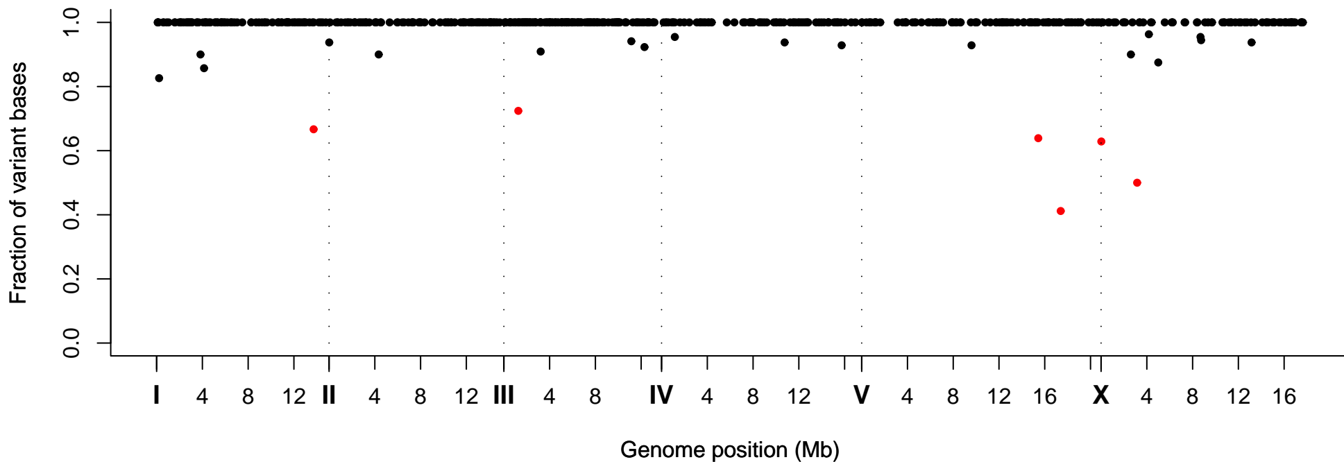
Fraction of Variant Bases at Position, Strain VC40754
