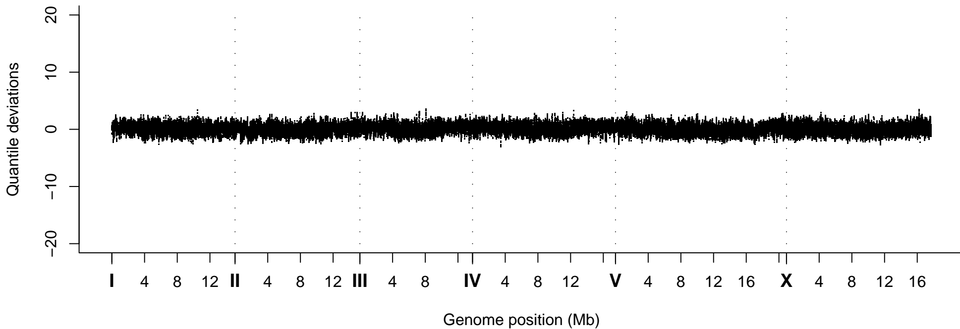
Quantile Deviations, Strain VC40754
