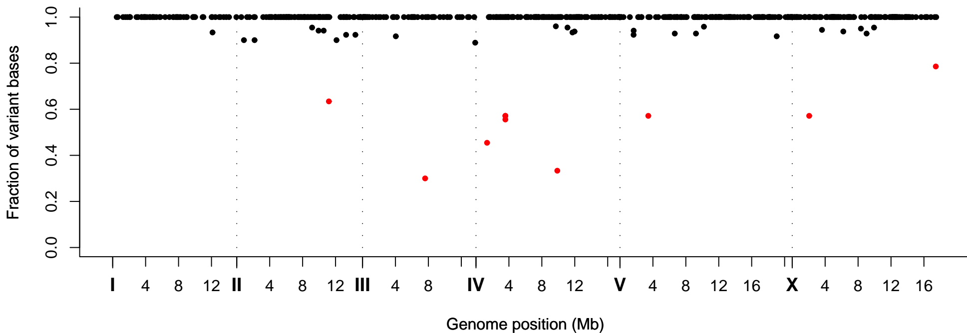
Fraction of Variant Bases at Position, Strain VC40760
