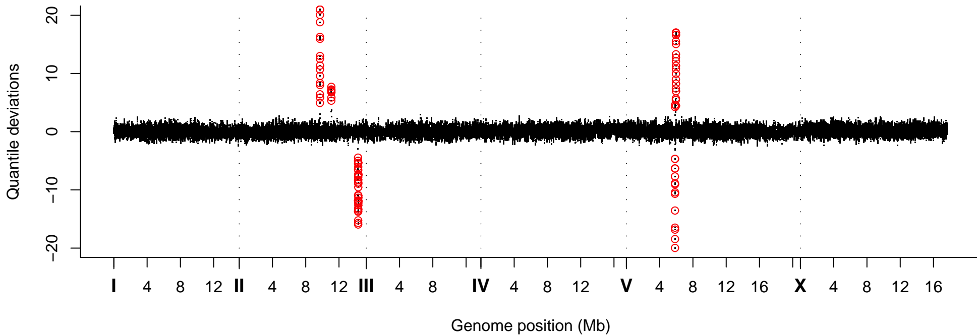
Quantile Deviations, Strain VC40760
