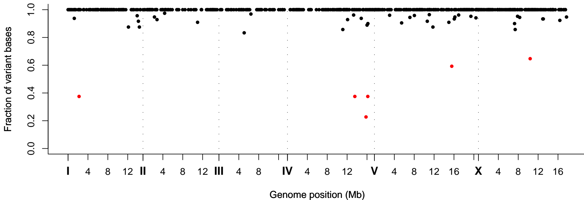
Fraction of Variant Bases at Position, Strain VC40764
