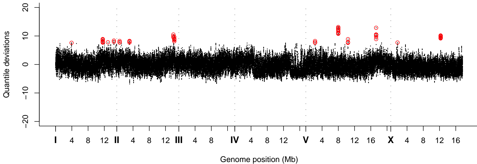
Quantile Deviations, Strain VC40764
