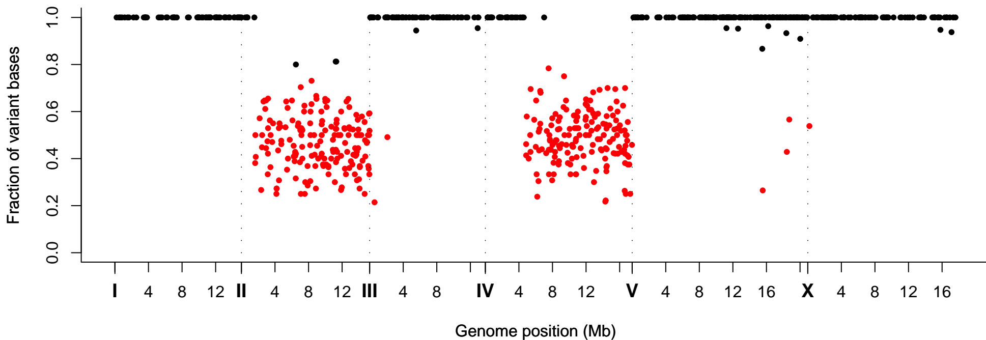
Fraction of Variant Bases at Position, Strain VC40767
