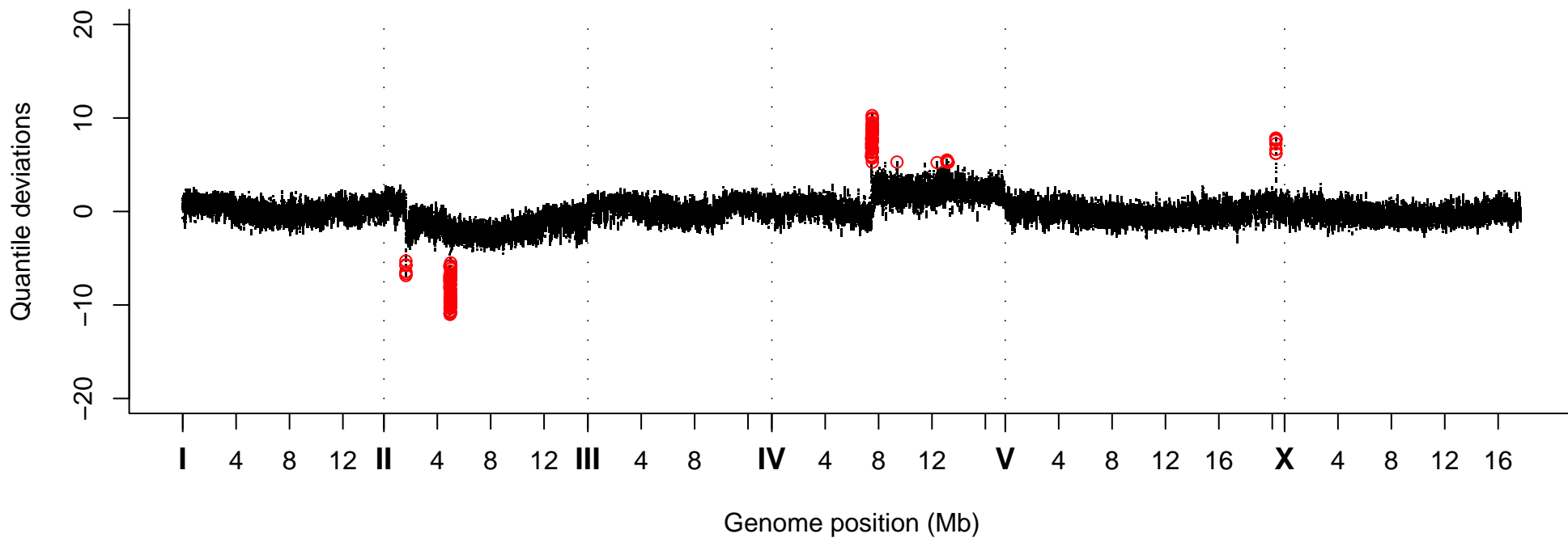
Quantile Deviations, Strain VC40767
