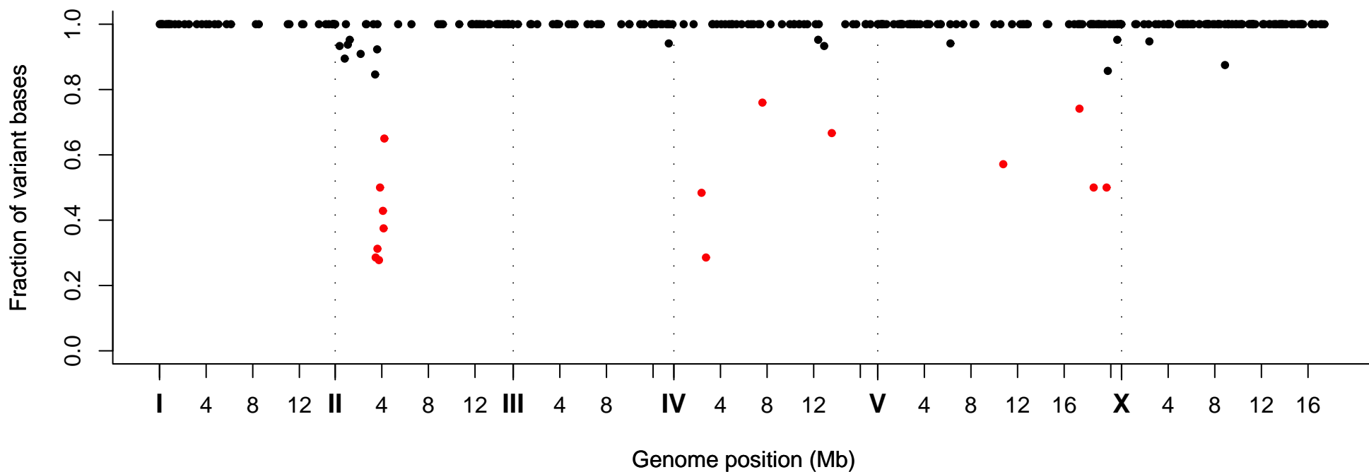
Fraction of Variant Bases at Position, Strain VC40768
