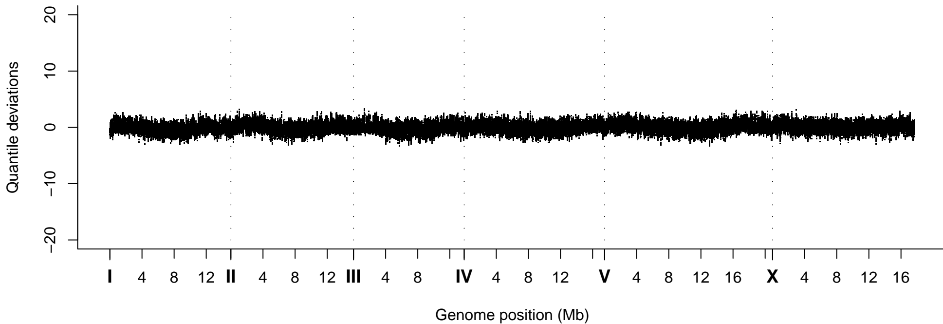
Quantile Deviations, Strain VC40768
