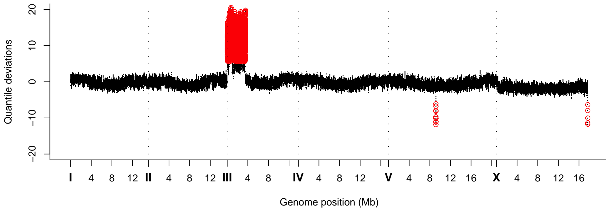
Quantile Deviations, Strain VC40772
