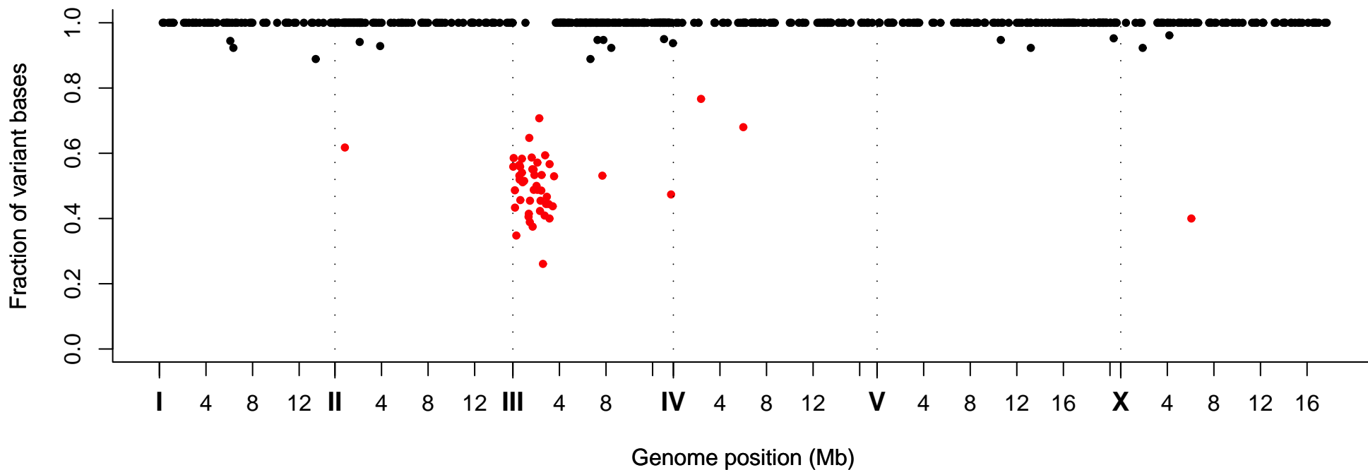
Fraction of Variant Bases at Position, Strain VC40772
