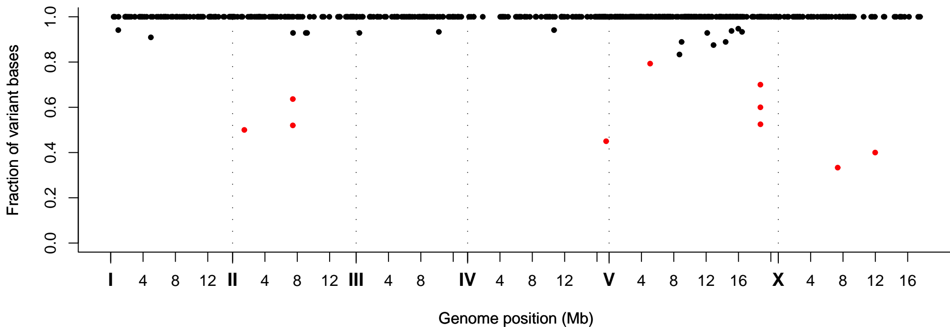
Fraction of Variant Bases at Position, Strain VC40773
