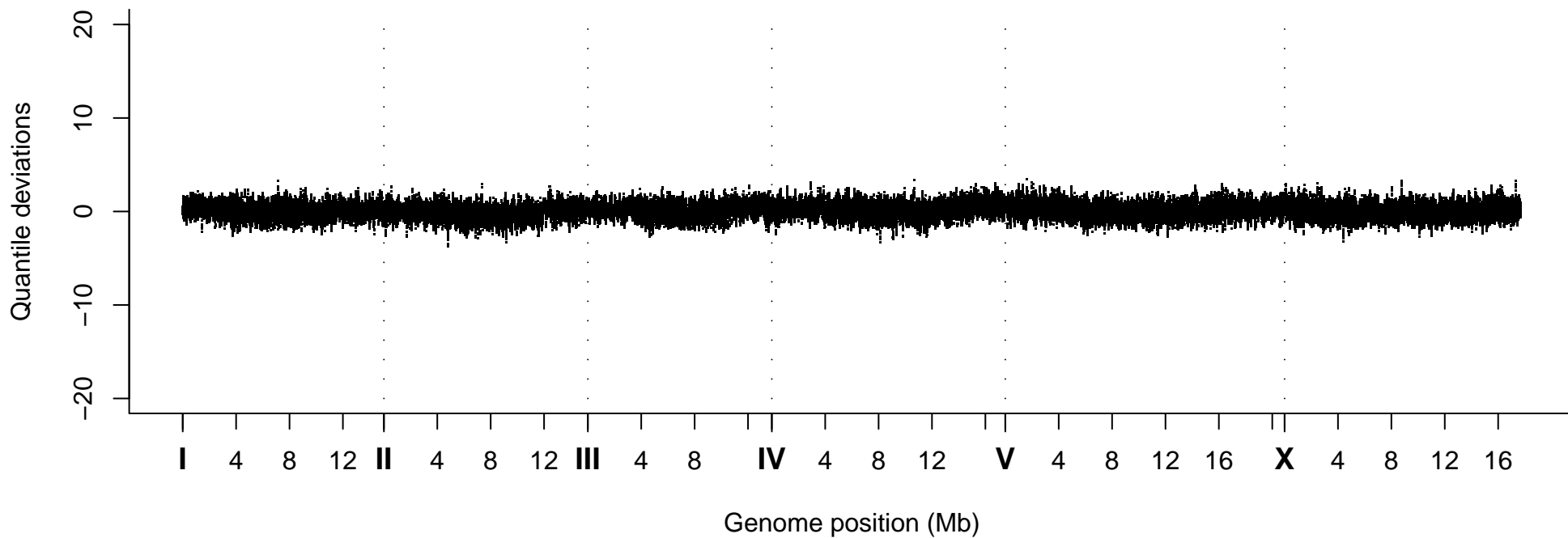
Quantile Deviations, Strain VC40773
