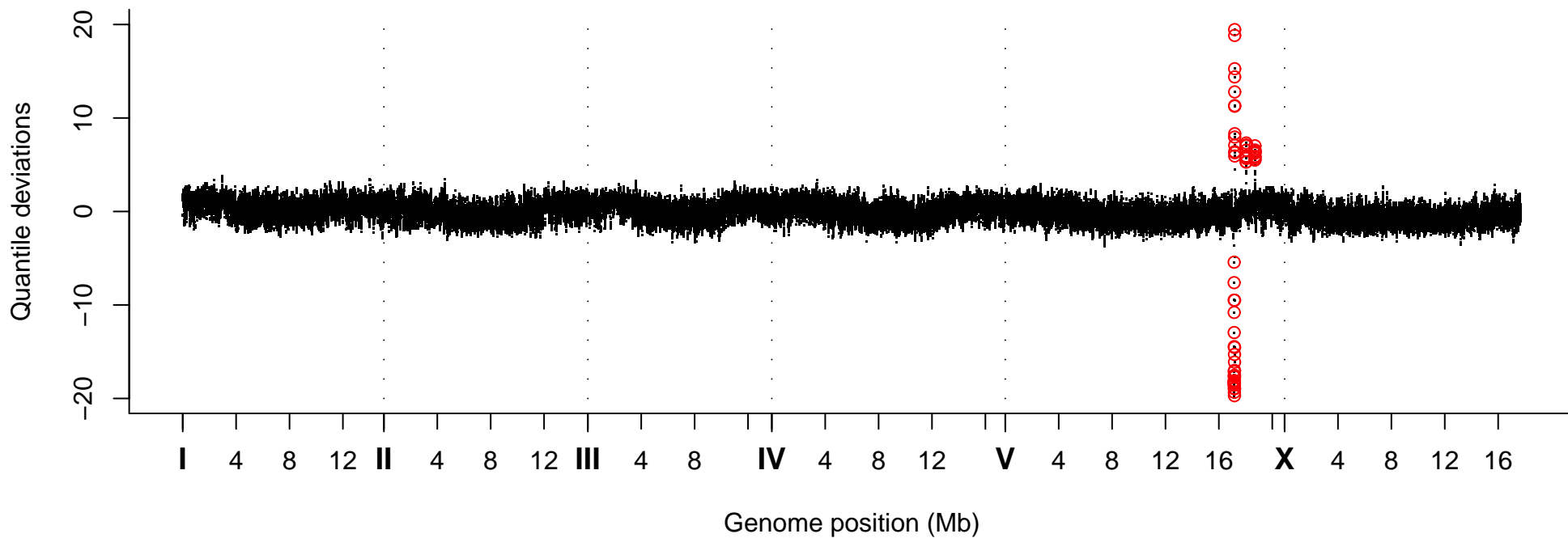
Quantile Deviations, Strain VC40777
