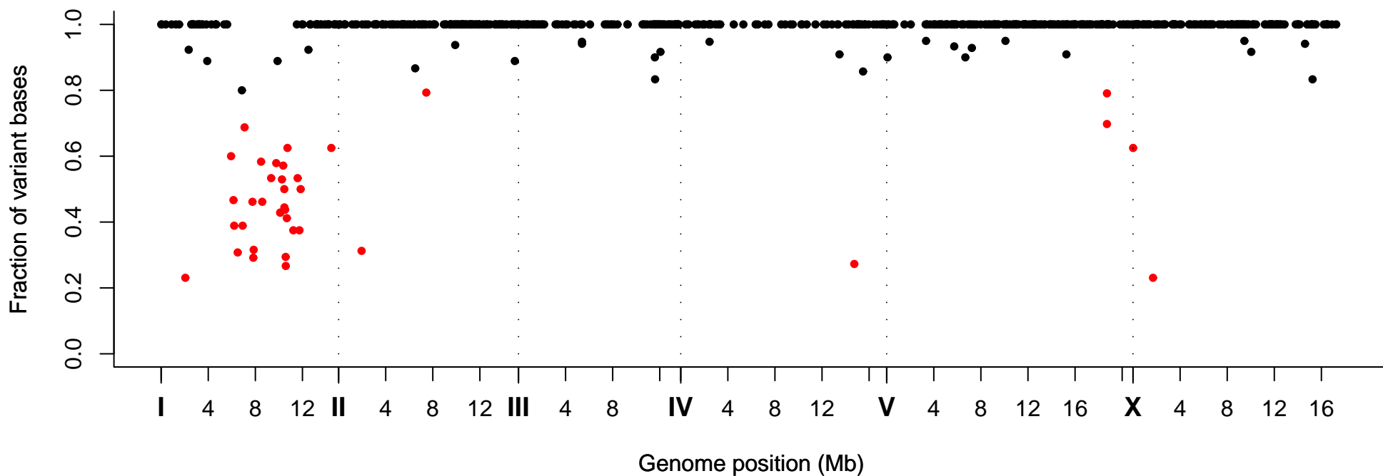
Fraction of Variant Bases at Position, Strain VC40777
