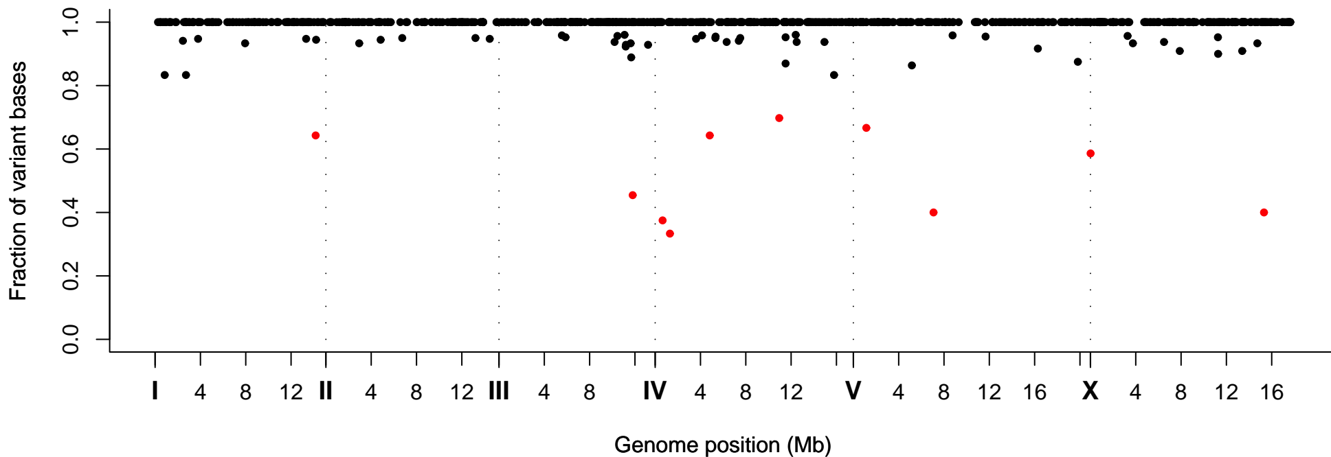
Fraction of Variant Bases at Position, Strain VC40799
