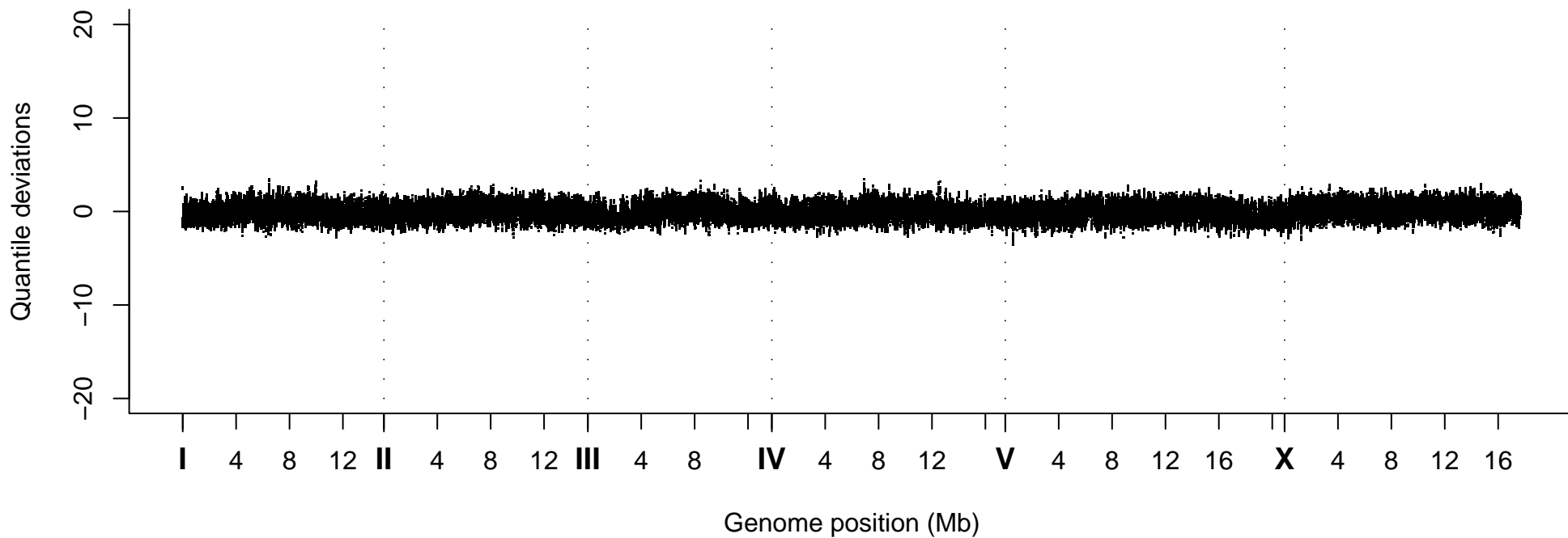
Quantile Deviations, Strain VC40799
