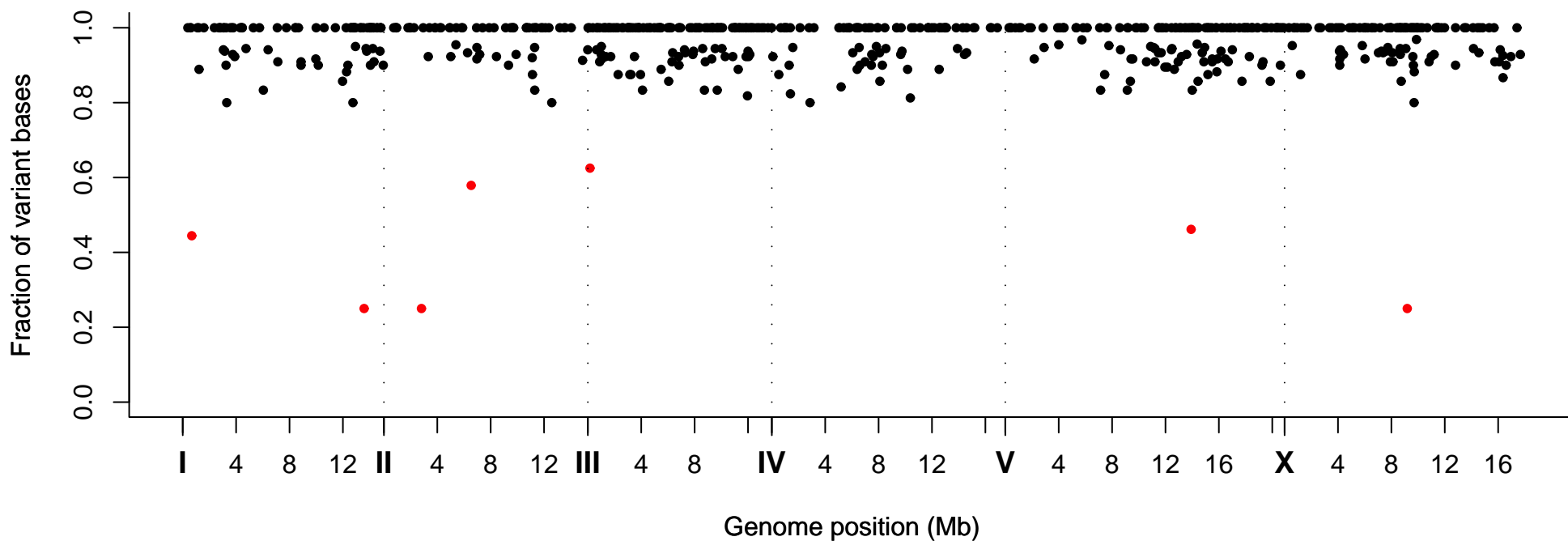
Fraction of Variant Bases at Position, Strain VC40800
