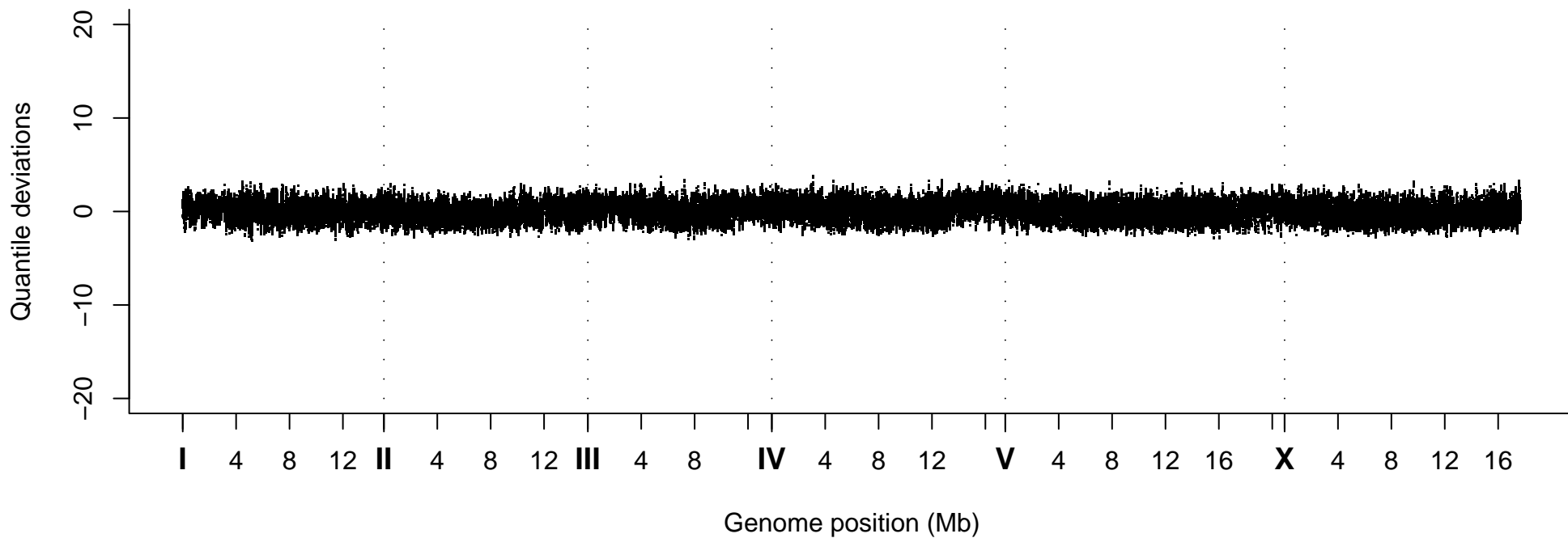
Quantile Deviations, Strain VC40800
