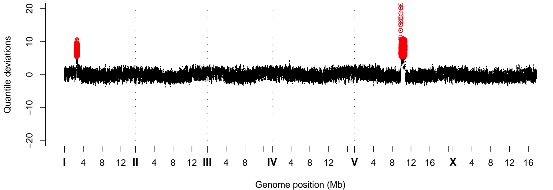
Quantile Deviations, Strain VC40801
