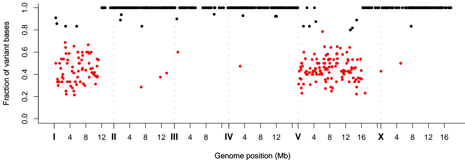
Fraction of Variant Bases at Position, Strain VC40801
