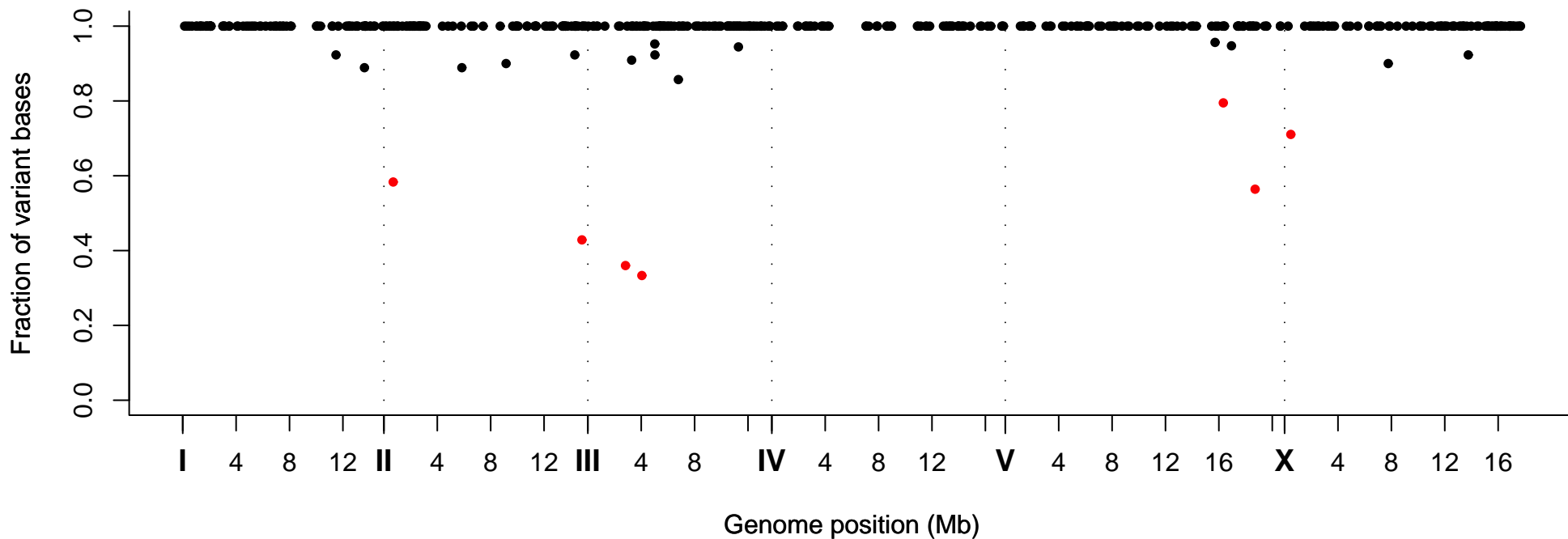
Fraction of Variant Bases at Position, Strain VC40806
