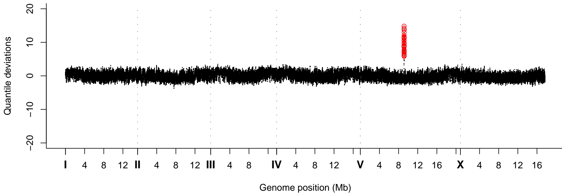
Quantile Deviations, Strain VC40806
