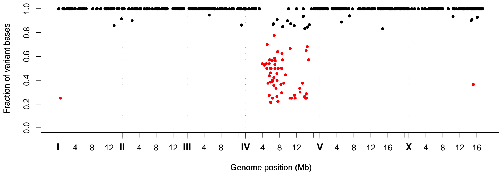
Fraction of Variant Bases at Position, Strain VC40818
