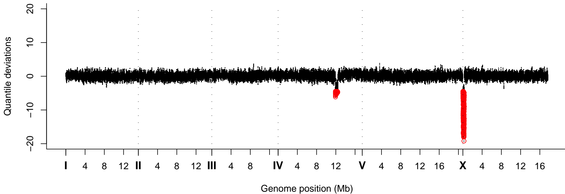
Quantile Deviations, Strain VC40818
