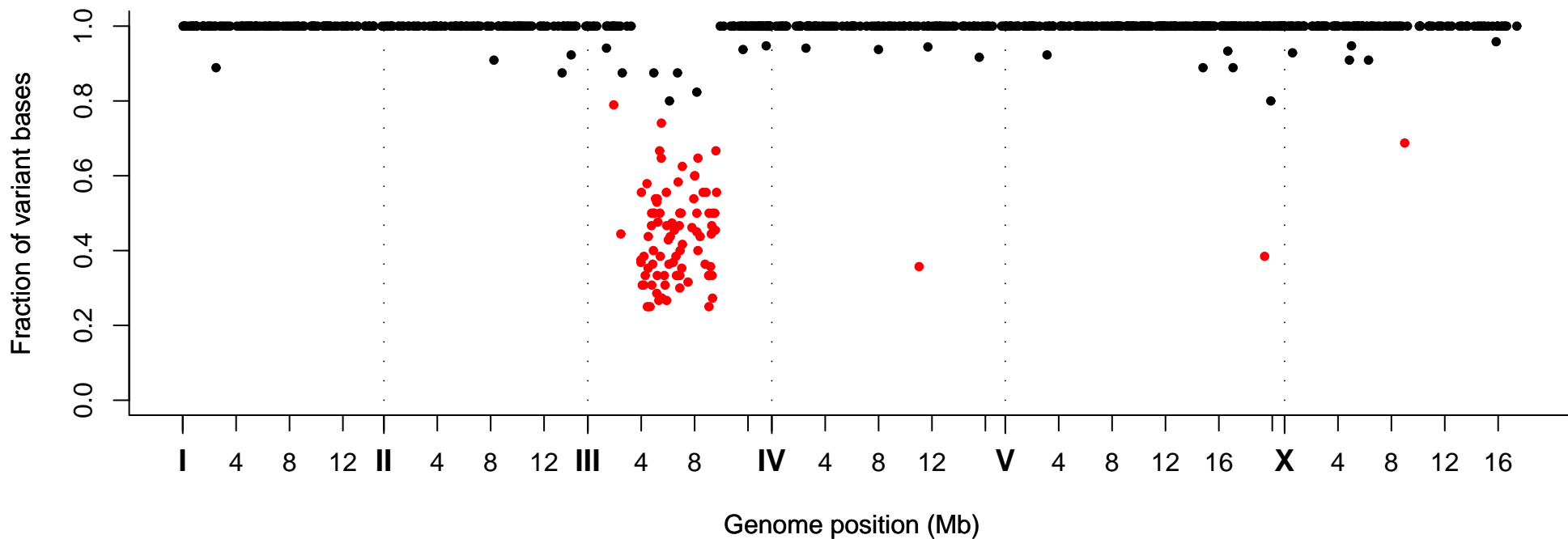
Fraction of Variant Bases at Position, Strain VC40819
