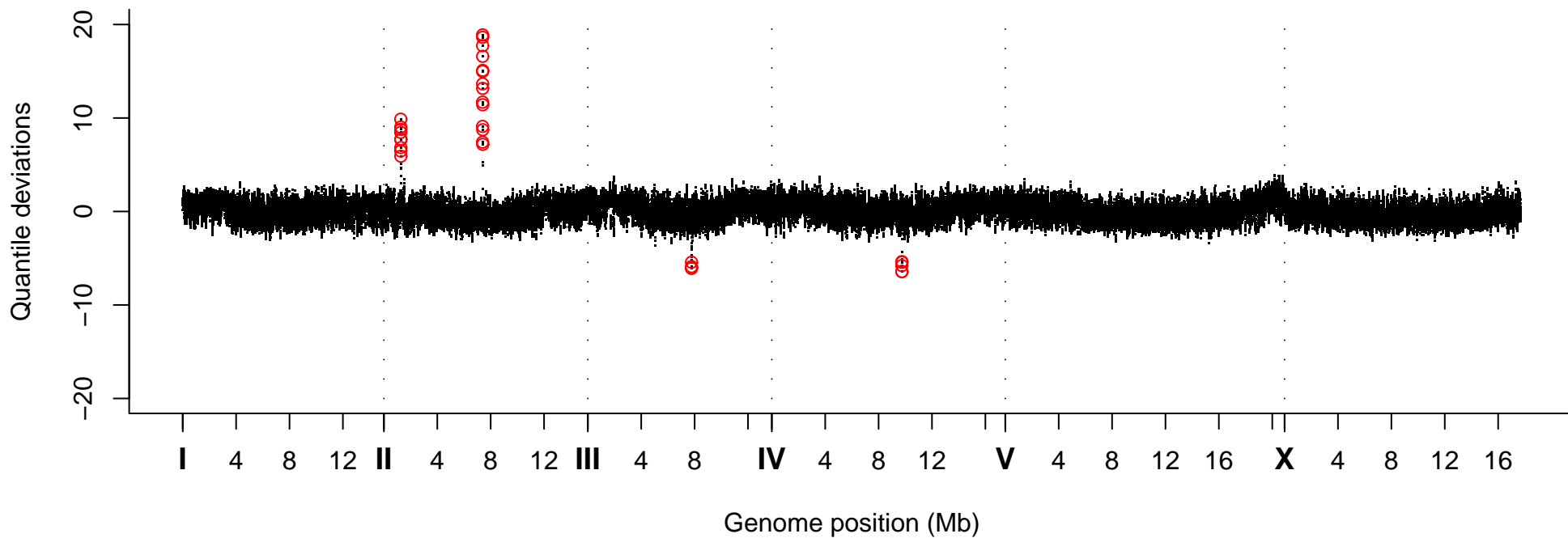
Quantile Deviations, Strain VC40819
