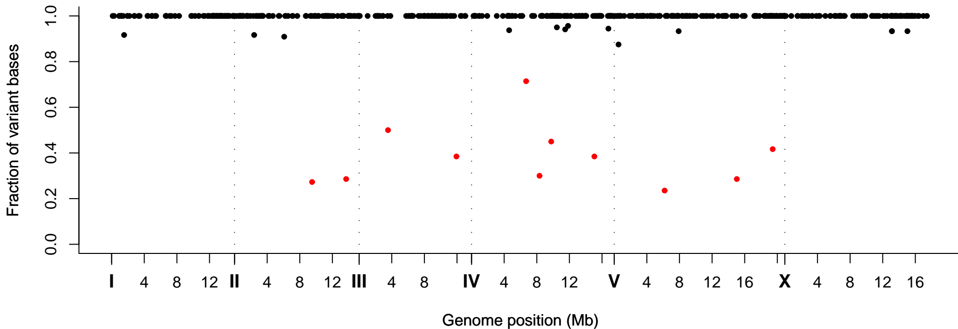
Fraction of Variant Bases at Position, Strain VC40825
