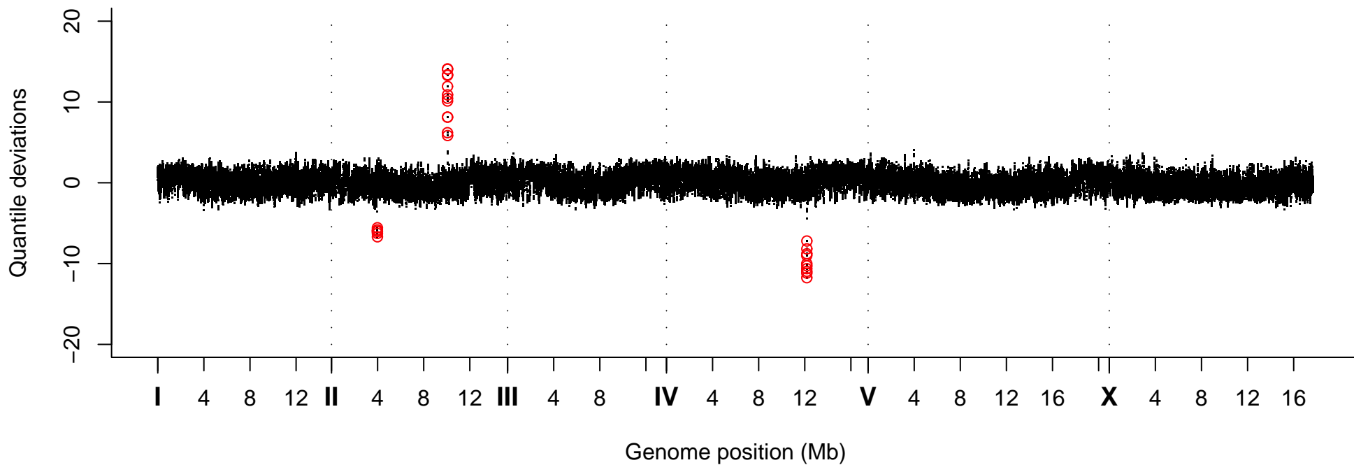
Quantile Deviations, Strain VC40825
