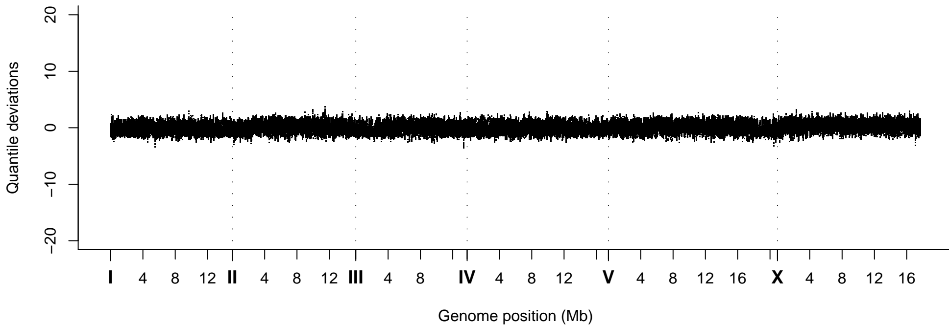
Quantile Deviations, Strain VC40827
