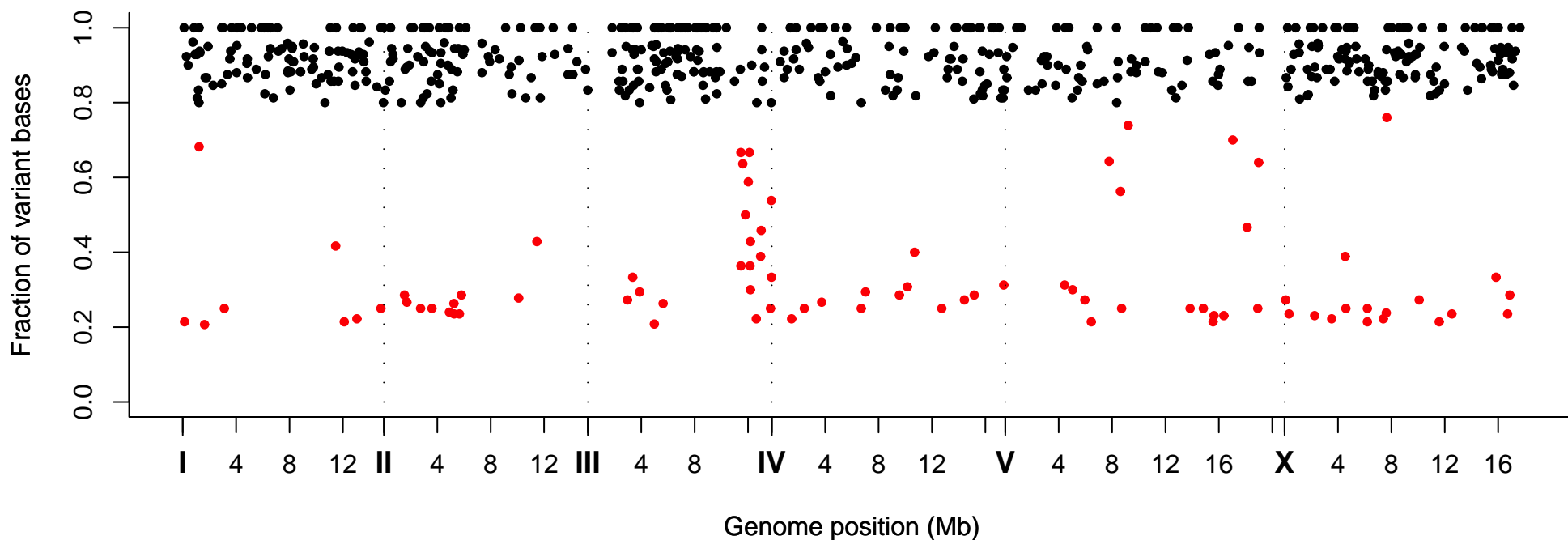
Fraction of Variant Bases at Position, Strain VC40827
