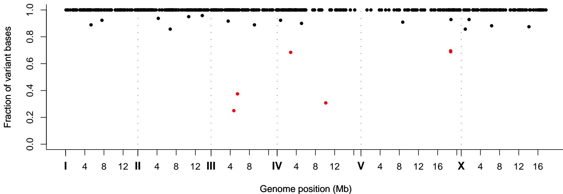
Fraction of Variant Bases at Position, Strain VC40828
