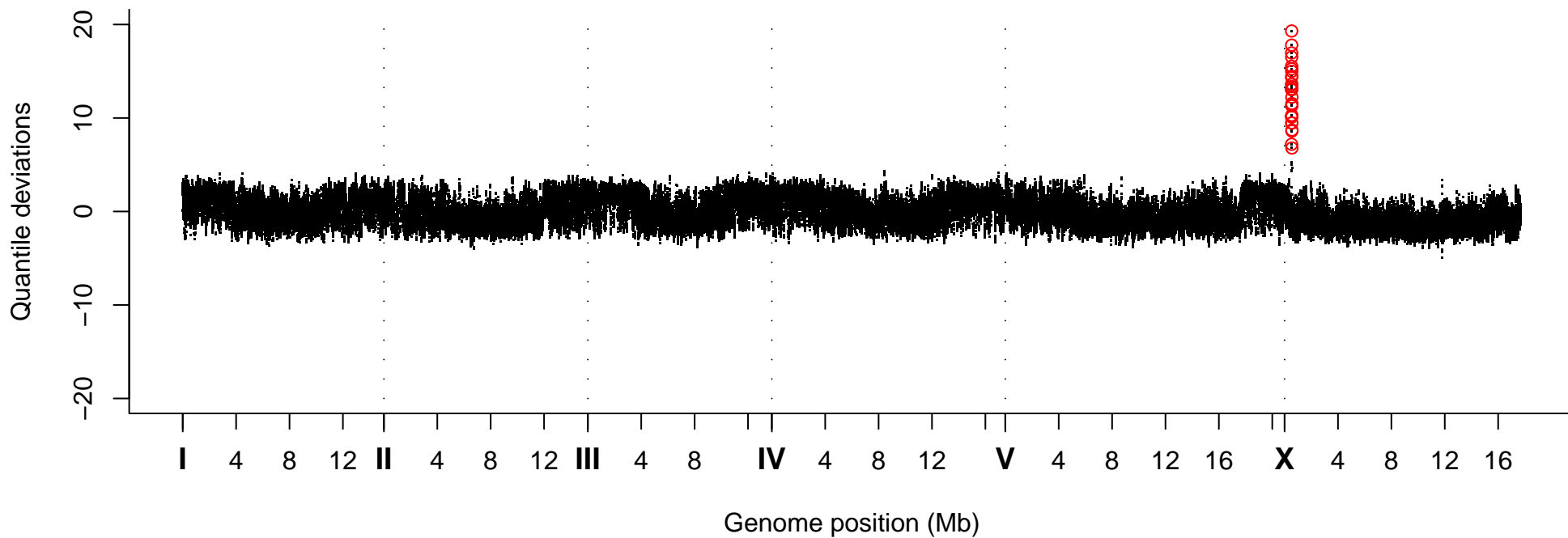
Quantile Deviations, Strain VC40828
