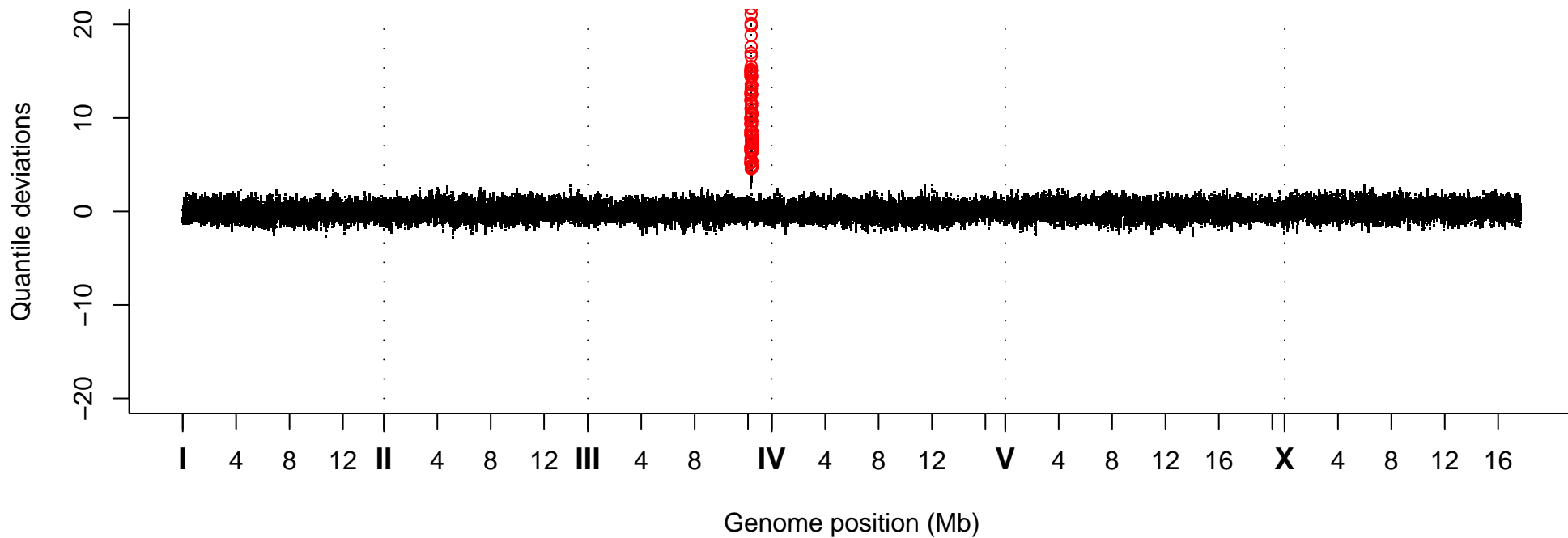
Quantile Deviations, Strain VC40830
