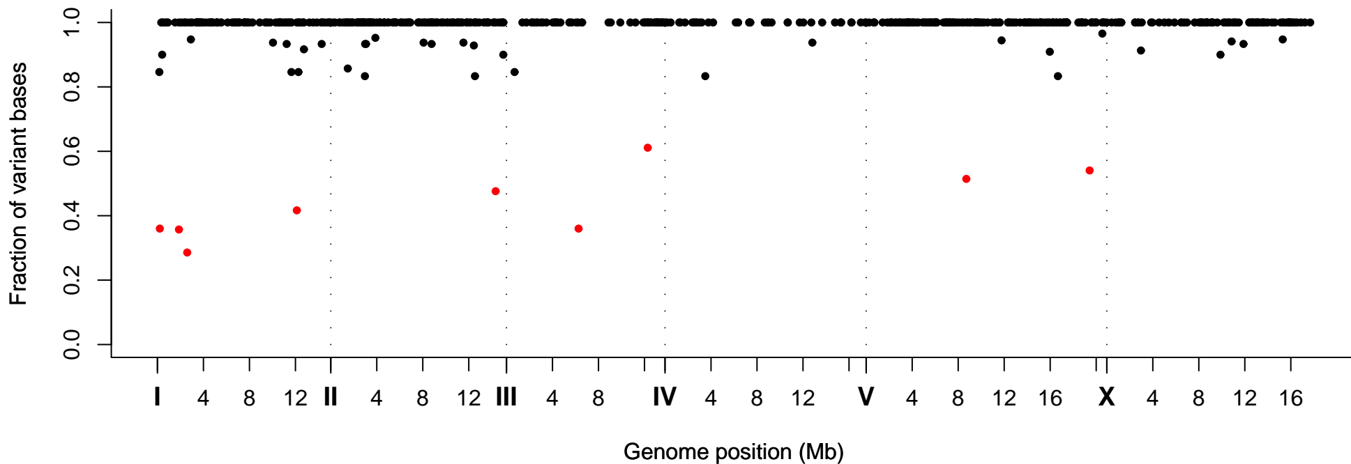
Fraction of Variant Bases at Position, Strain VC40830
