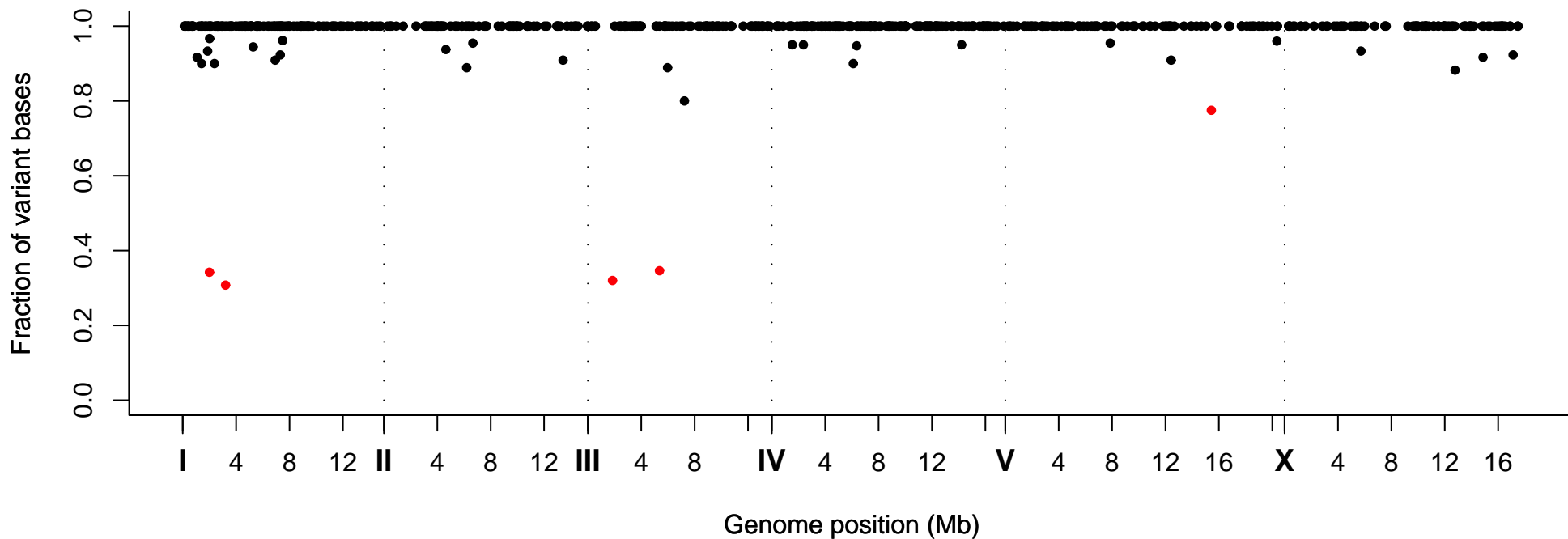
Fraction of Variant Bases at Position, Strain VC40833
