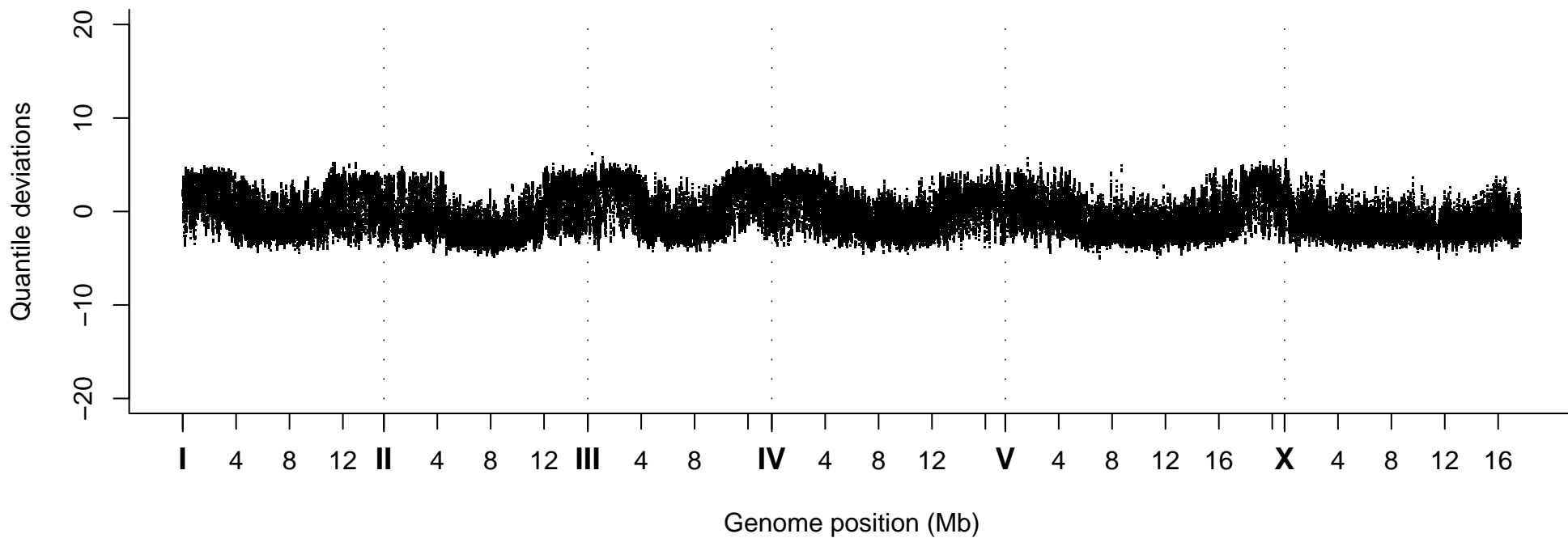
Quantile Deviations, Strain VC40833
