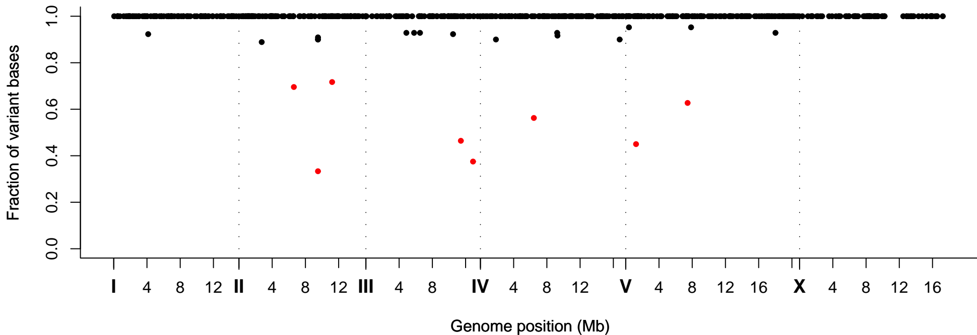
Fraction of Variant Bases at Position, Strain VC40836
