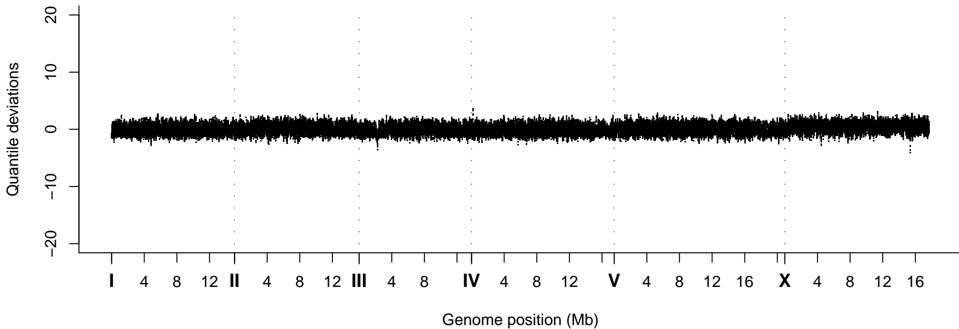
Quantile Deviations, Strain VC40836
