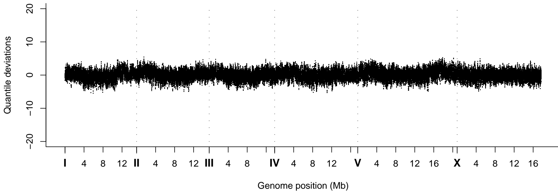
Quantile Deviations, Strain VC40850
