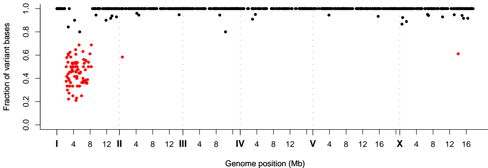
Fraction of Variant Bases at Position, Strain VC40850
