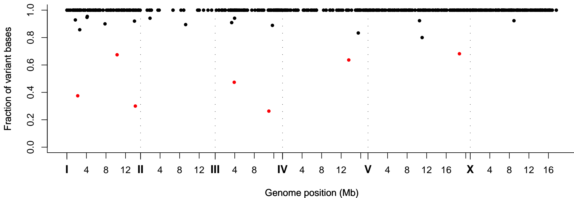
Fraction of Variant Bases at Position, Strain VC40854
