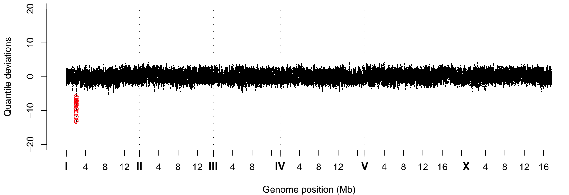
Quantile Deviations, Strain VC40854
