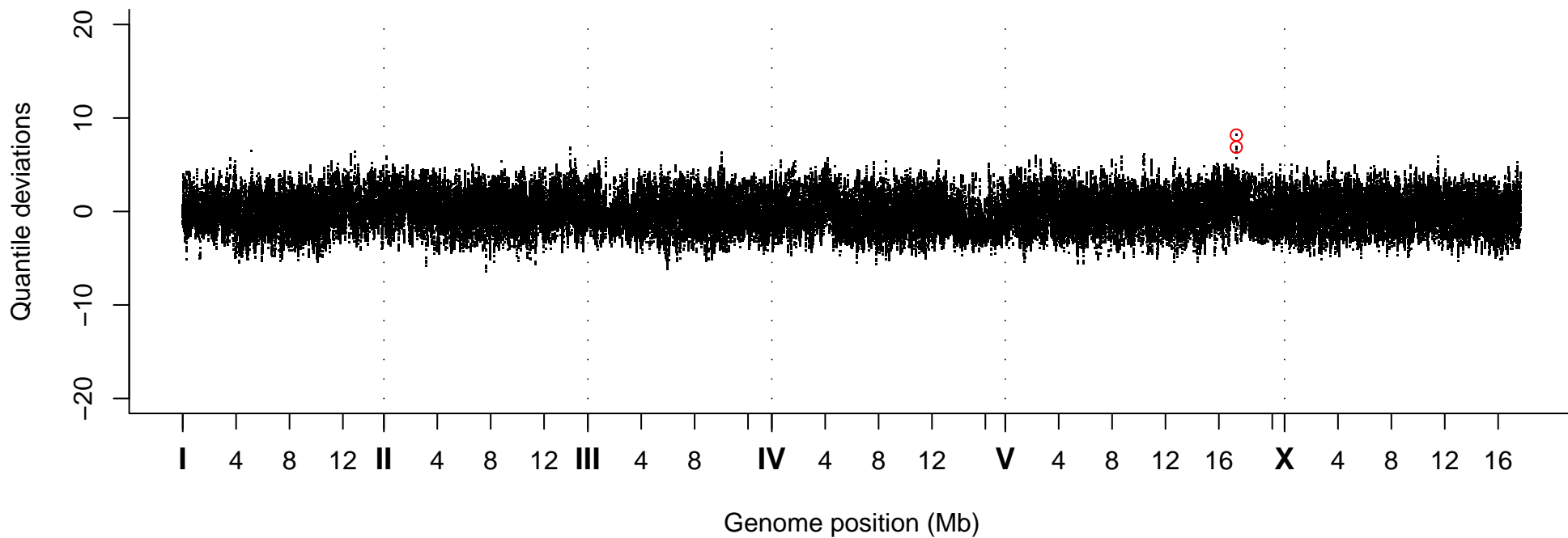
Quantile Deviations, Strain VC40857
