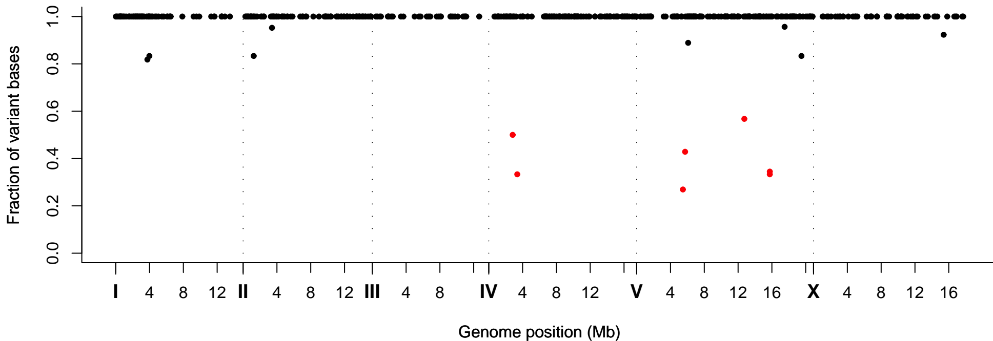
Fraction of Variant Bases at Position, Strain VC40857
