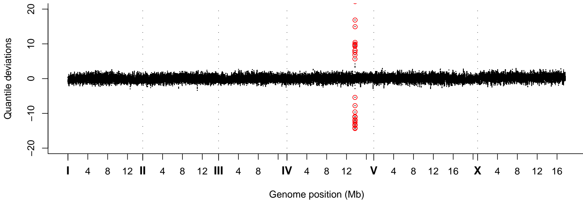
Quantile Deviations, Strain VC40858
