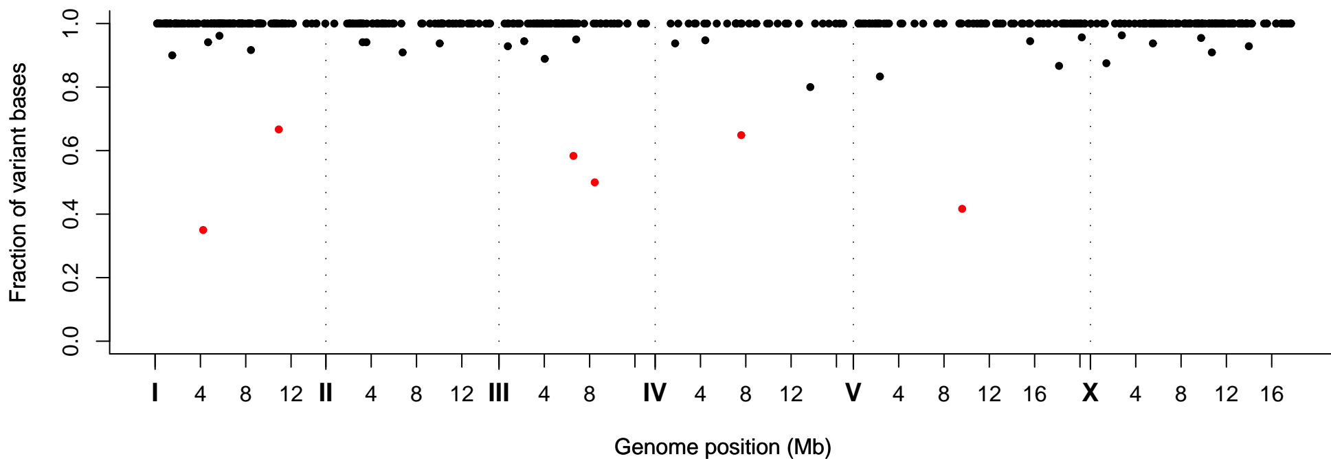
Fraction of Variant Bases at Position, Strain VC40858
