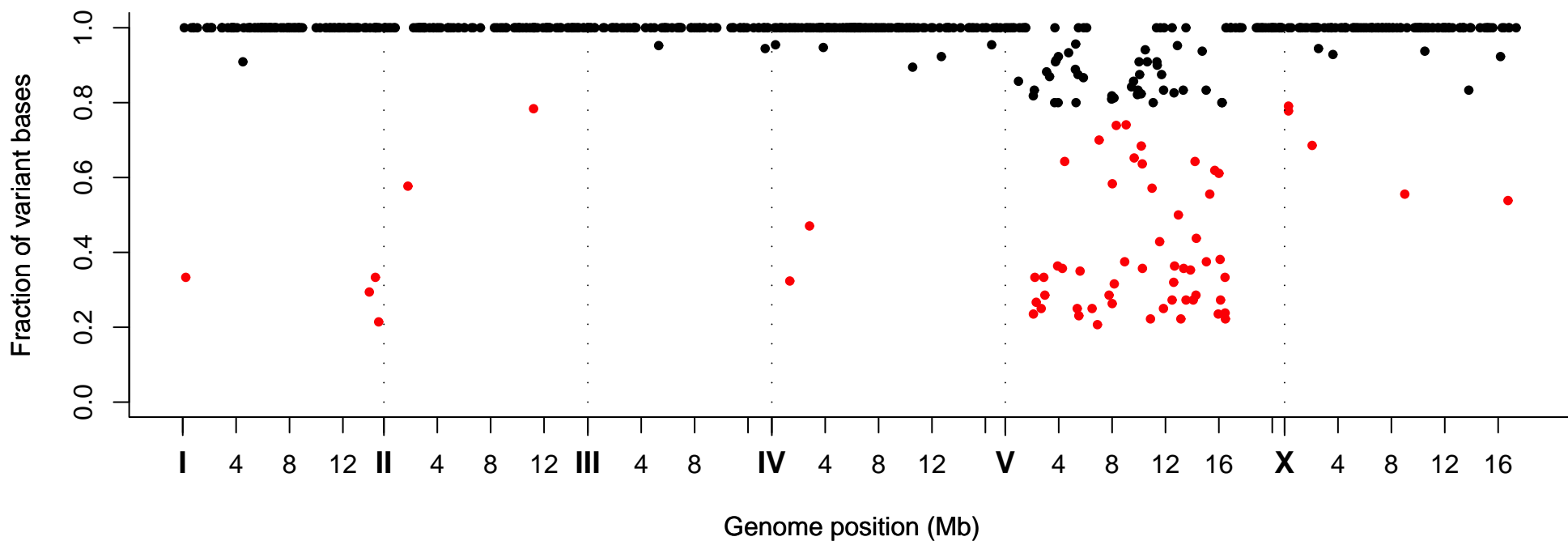
Fraction of Variant Bases at Position, Strain VC40859
