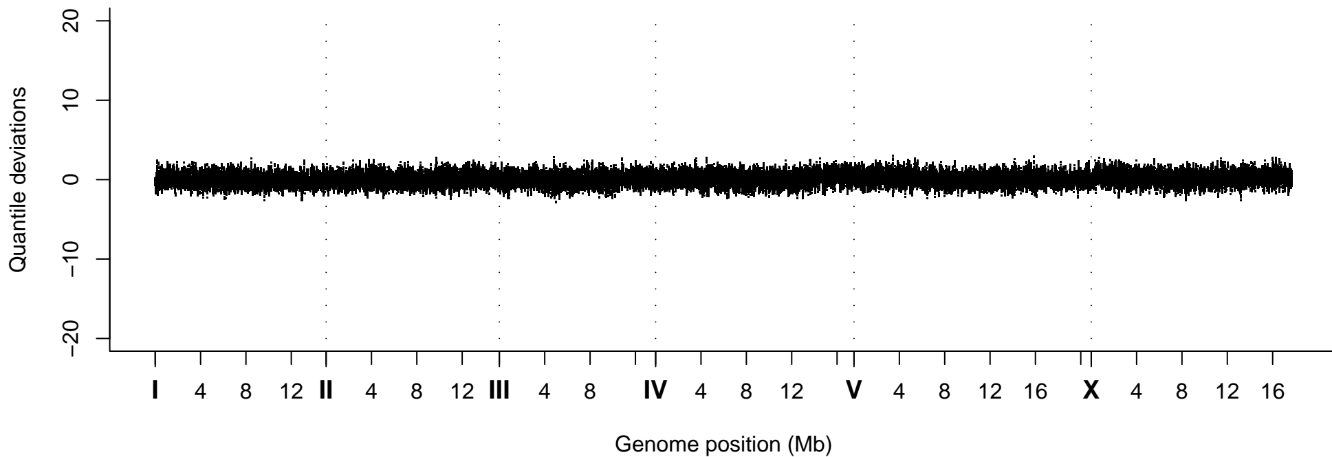
Quantile Deviations, Strain VC40859
