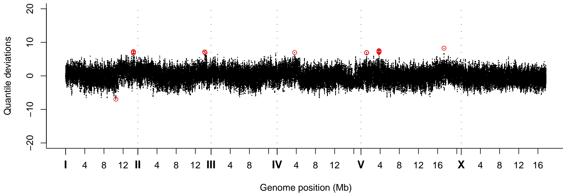
Quantile Deviations, Strain VC40864
