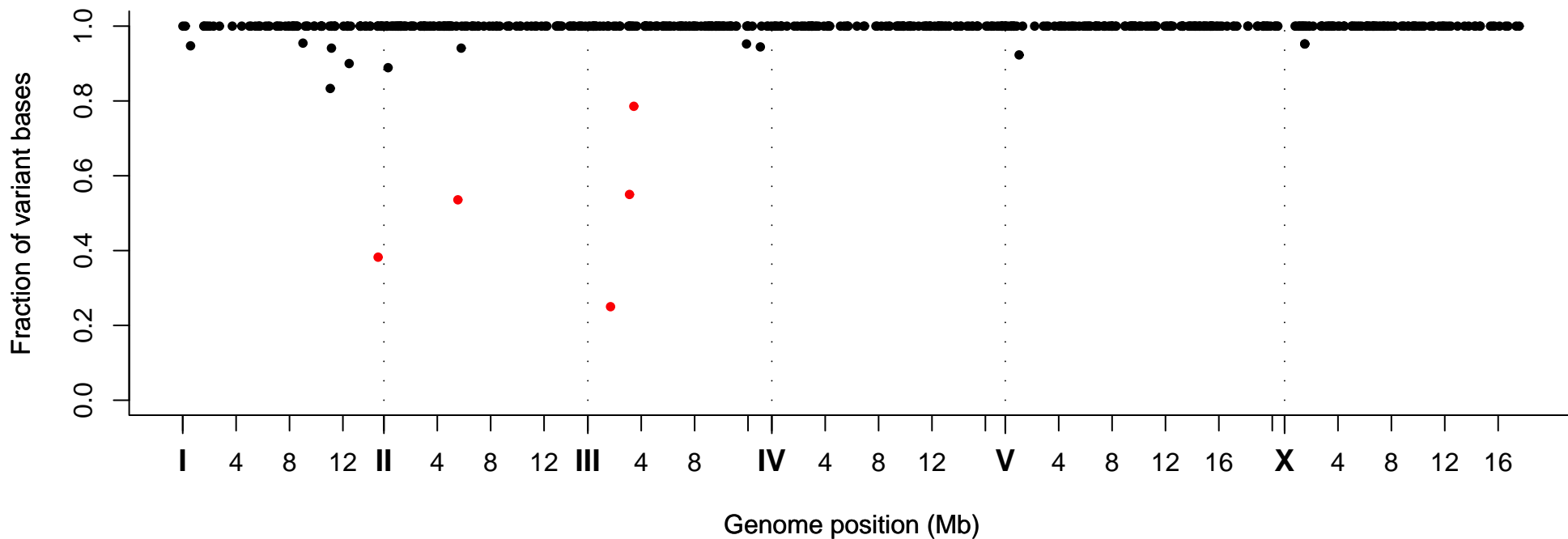
Fraction of Variant Bases at Position, Strain VC40864
