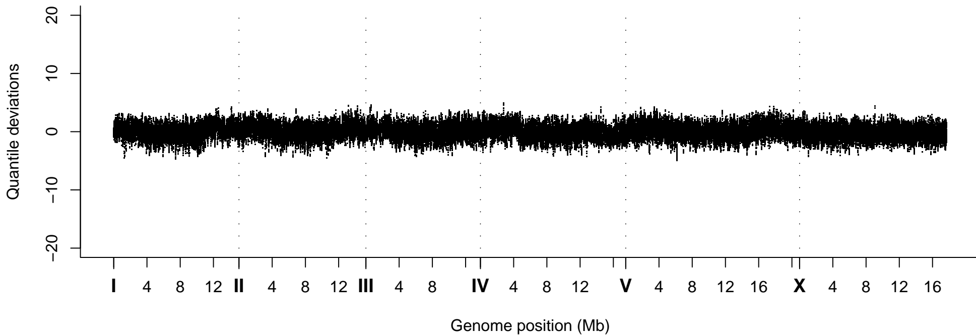
Quantile Deviations, Strain VC40869
