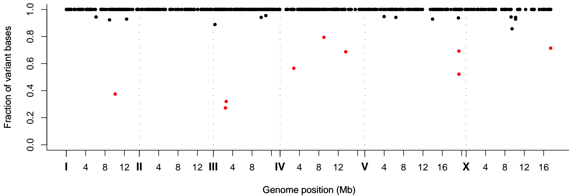
Fraction of Variant Bases at Position, Strain VC40869
