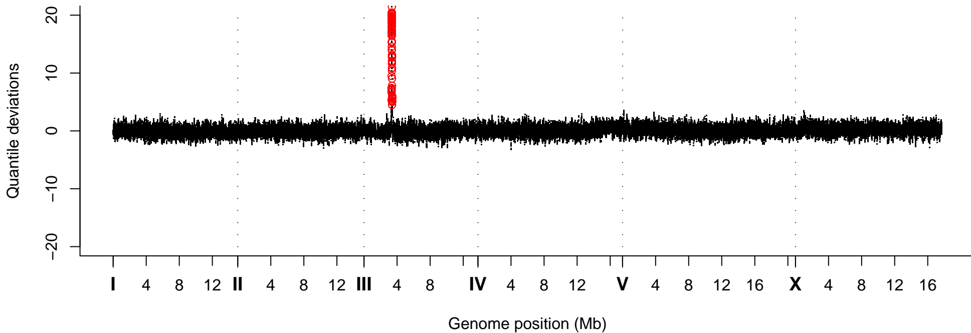
Quantile Deviations, Strain VC40874
