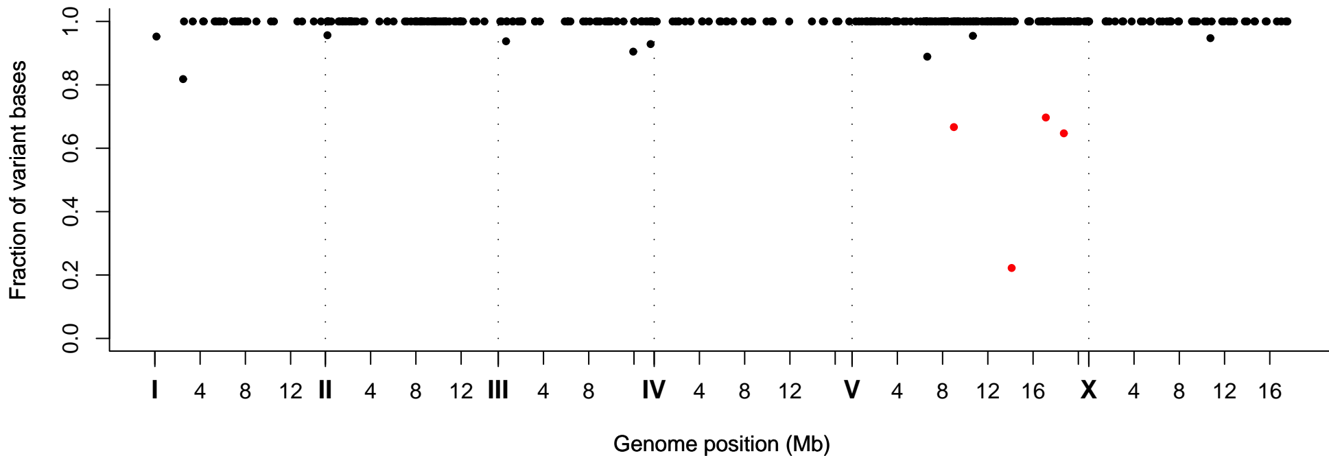
Fraction of Variant Bases at Position, Strain VC40874
