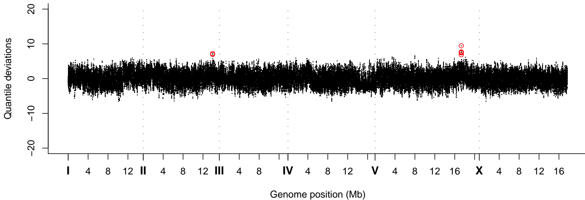
Quantile Deviations, Strain VC40877
