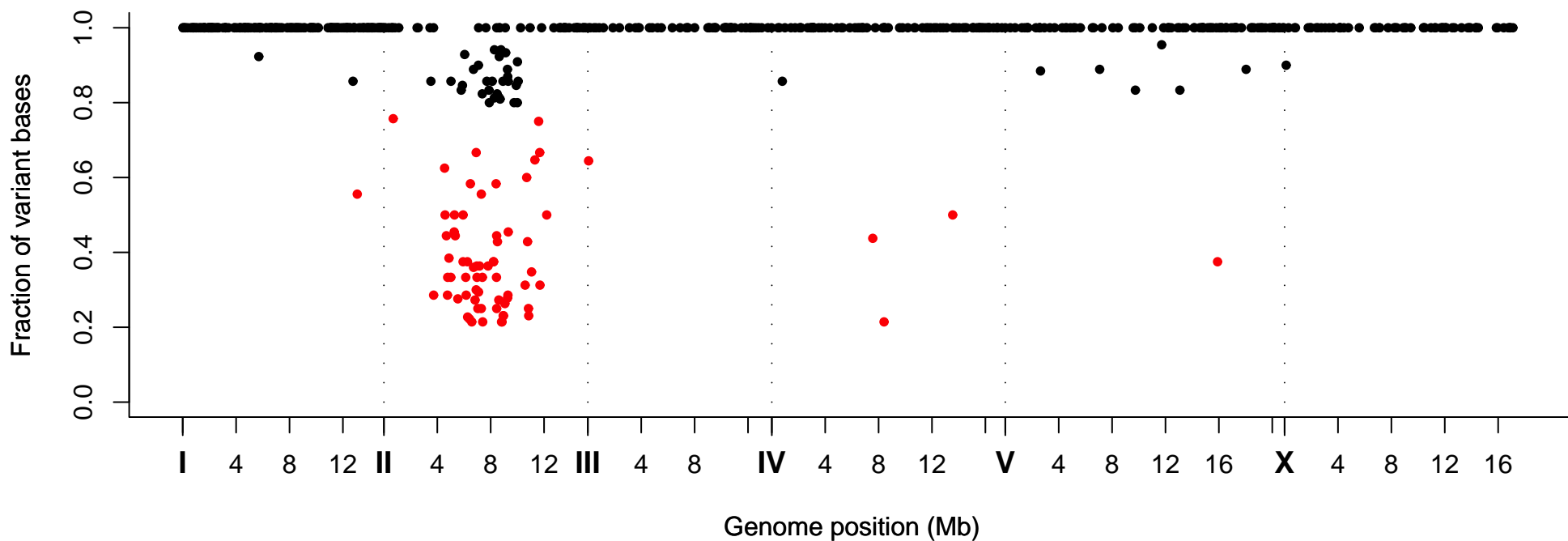
Fraction of Variant Bases at Position, Strain VC40877
